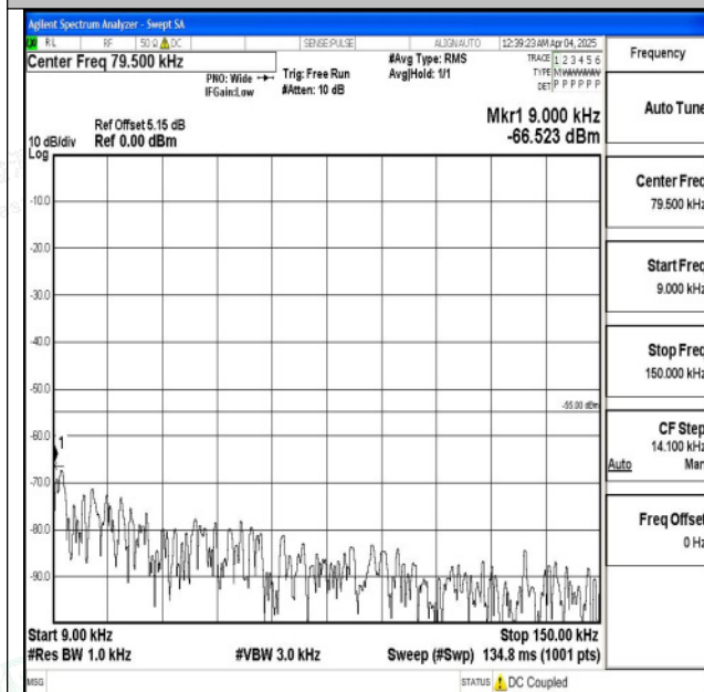
Band7_5MHz_QPSK_20775_1RB#0_0.009~0.15_0.009~0.15
