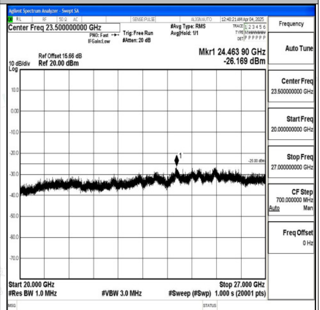
Band7_5MHz_16QAM_20775_1RB#0_20000~27000_20000~27000
