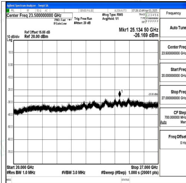
Band7_10MHz_QPSK_21400_1RB#0_20000~27000_2000~27000
