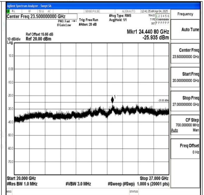
Band7_5MHz_16QAM_21100_1RB#0_20000~27000_20 000~27000
