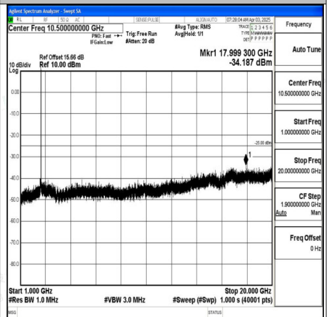
Band7_10MHz_QPSK_21400_1RB#0_1000~20000_1000~20000
