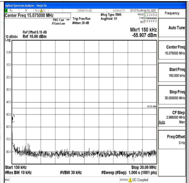
Band7_10MHz_QPSK_21400_1RB#0_0.15~30_0.15~30
