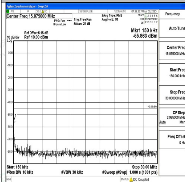
Band7_10MHz_16QAM_21400_1RB#0_0.15~30_0.15~30
