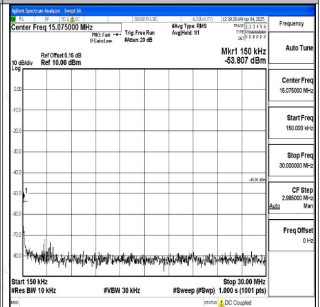
Band7_5MHz_QPSK_20775_1RB#0_0.15~30_0.15~30
