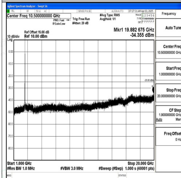
Band7_10MHz_16QAM_21100_1RB#0_1000~20000_10 00~20000
