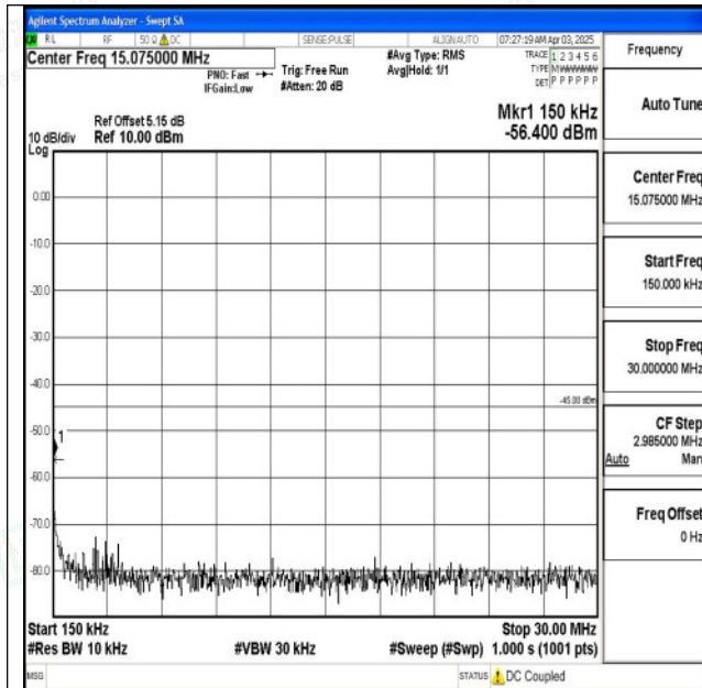
Band7_10MHz_16QAM_21100_1RB#0_0.15~30_0.15~3 0
