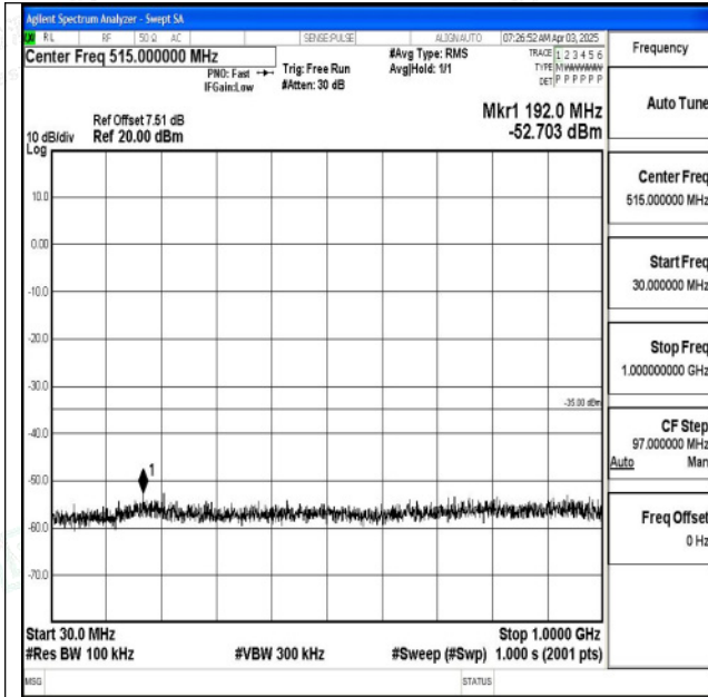
Band7_10MHz_QPSK_21100_1RB#0_30~1000_30~1000 0
