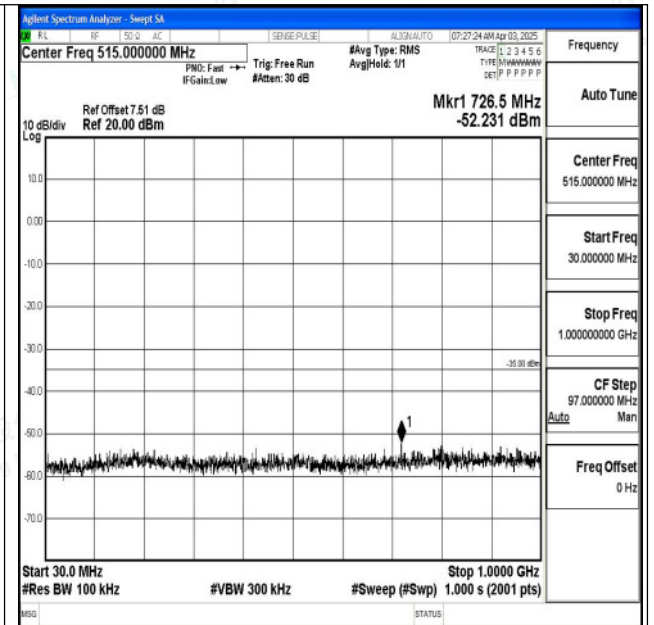
Band7_10MHz_16QAM_21100_1RB#0_30~1000_30~10 00
