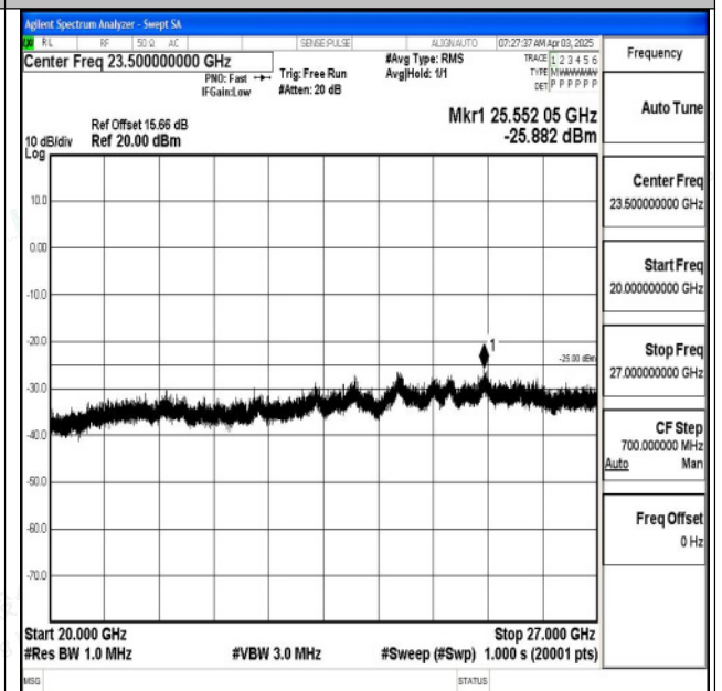
Band7_10MHz_16QAM_21100_1RB#0_20000~27000_2 0000~27000
