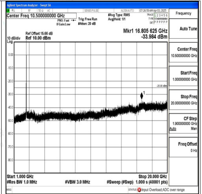
Band7_10MHz_QPSK_21100_1RB#0_1000~20000_1000~20000 0~20000
