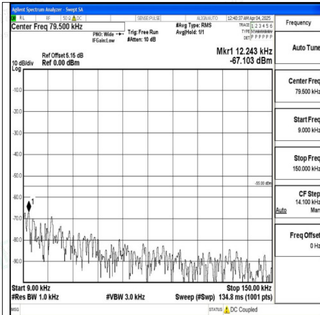
Band7_5MHz_QPSK_21100_1RB#0_0.009~0.15_0.009~0.15
