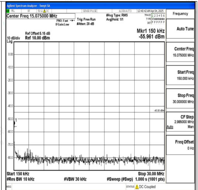
Band7_5MHz_QPSK_21100_1RB#0_0.15~30_0.15~30
