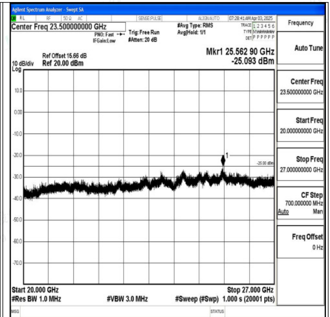
Band7_10MHz_16QAM_21400_1RB#0_20000~27000_20000~27000
