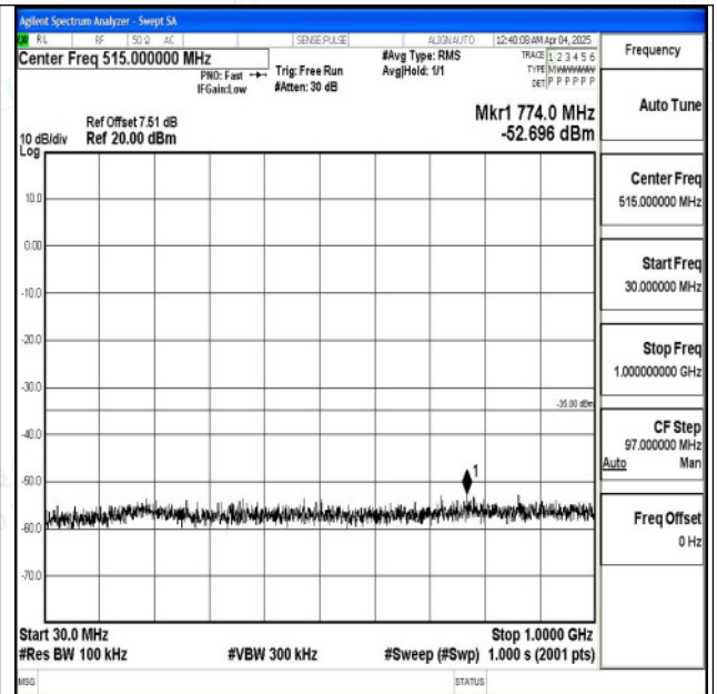
Band7_5MHz_16QAM_20775_1RB#0_30~1000_30~1000 0
