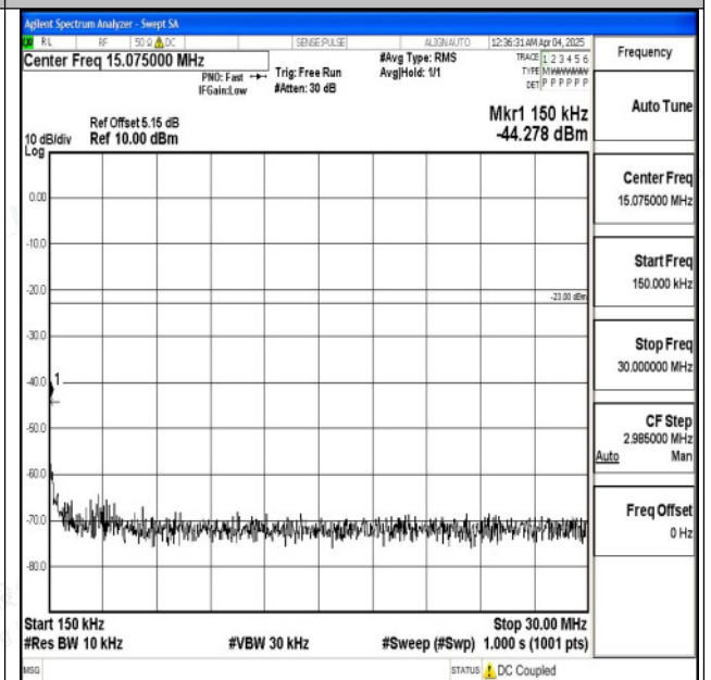
Band5_10MHz_QPSK_20600_1RB#0_0.15~30_0.15~30
