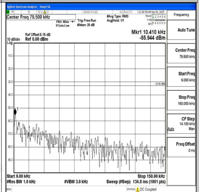
Band5_10MHz_16QAM_20600_1RB#0_0.009~0.15_0.0 09~0.15
