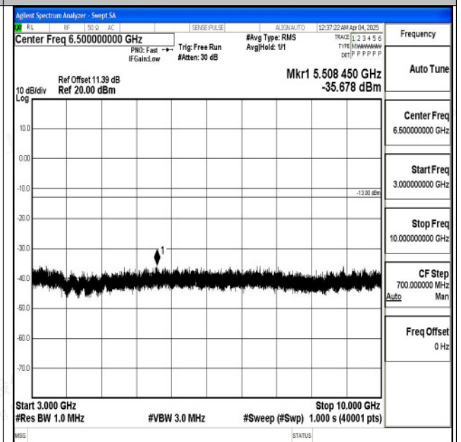
Band5_10MHz_16QAM_20600_1RB#0_3000~10000_30
