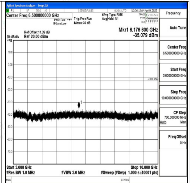
Band5_10MHz_16QAM_20525_1RB#0_3000~10000_30 00~10000
