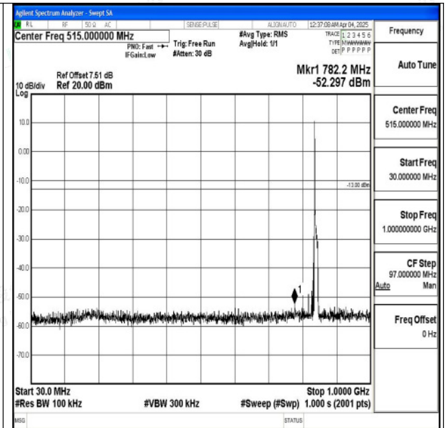
Band5_10MHz_16QAM_20600_1RB#0_30~1000_30~10
