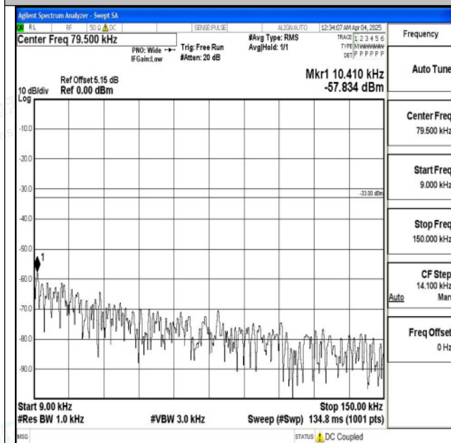
Band5_10MHz_QPSK_20450_1RB#0_0.009~0.15_0.009 ~0.15
