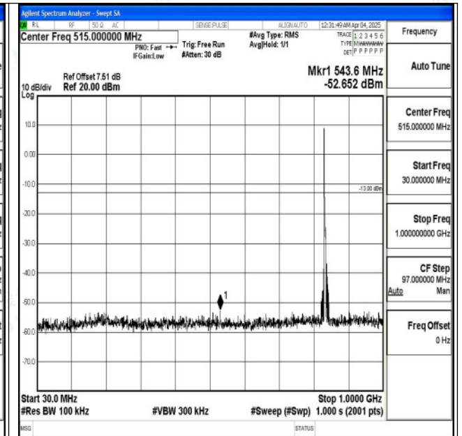
Band5_5MHz_16QAM_20525_1RB#0_30~1000_30~1000
