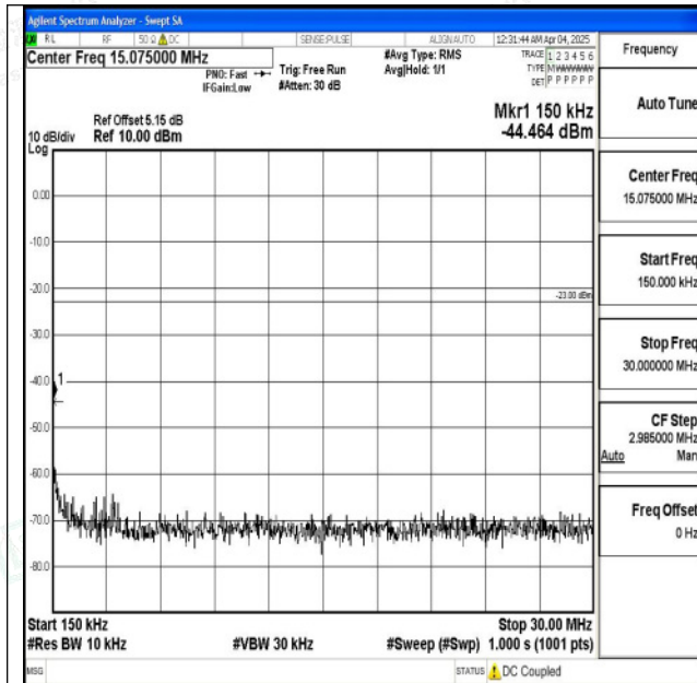
Band5_5MHz_16QAM_20525_1RB#0_0.15~30_0.15~30
