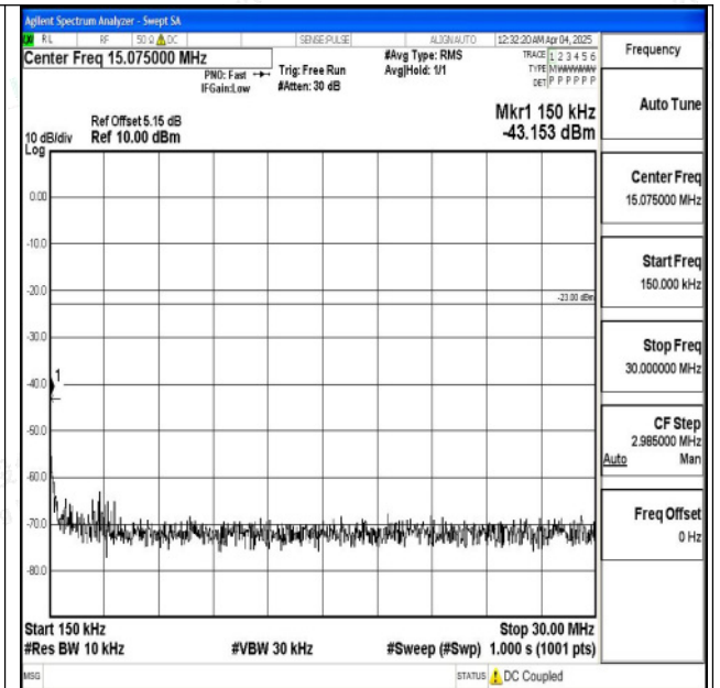
Band5_5MHz_QPSK_20625_1RB#0_0.15~30_0.15~30
