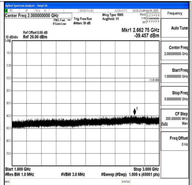
Band5_5MHz_QPSK_20525_1RB#0_1000~3000_1000~3000
