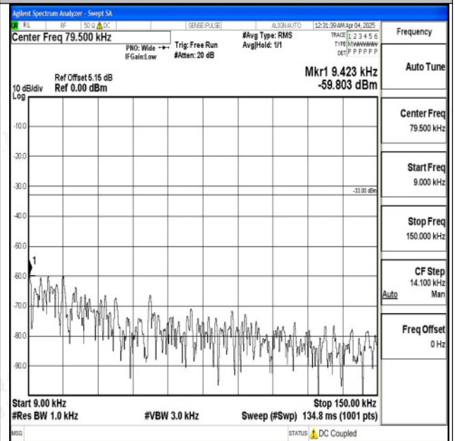
Band5_5MHz_16QAM_20525_1RB#0_0.009~0.15_0.009~0.15
