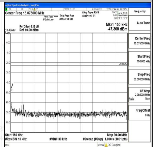
Band5_10MHz_QPSK_20450_1RB#0_0.15~30_0.15~30
