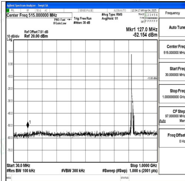
Band5_10MHz_QPSK_20450_1RB#0_30~1000_30~1000 0
