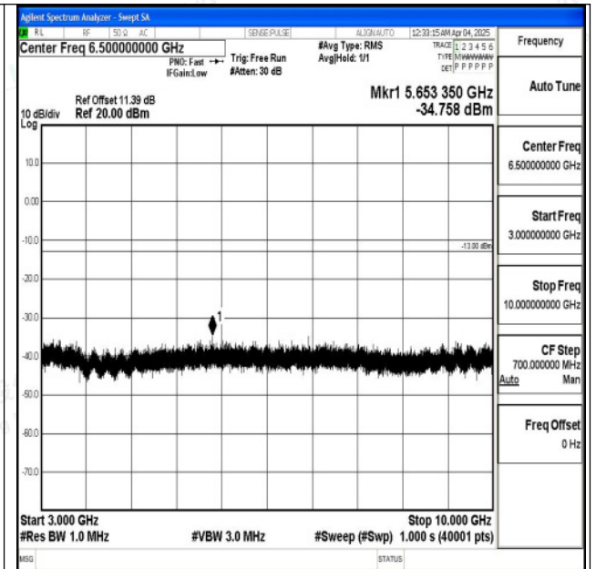
Band5_5MHz_16QAM_20625_1RB#0_3000~10000_300 0~10000
