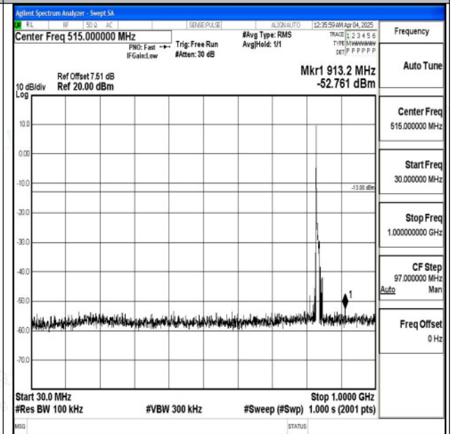
Band5_10MHz_16QAM_20525_1RB#0_30~1000_30~10 00
