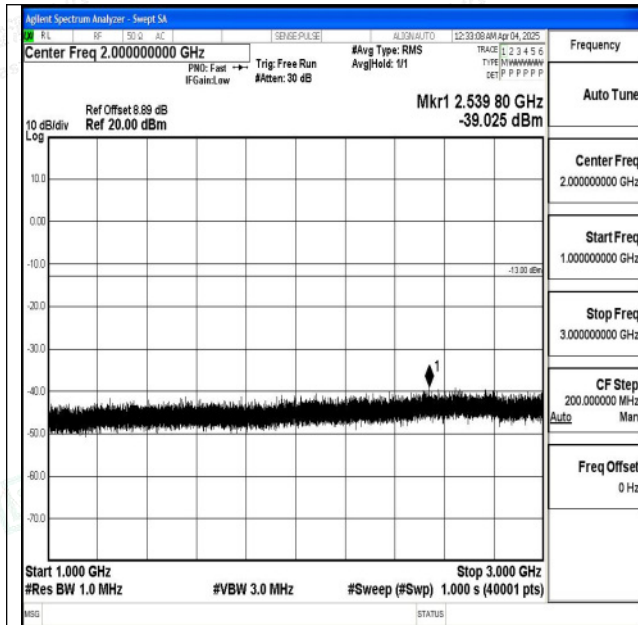
Band5_5MHz_16QAM_20625_1RB#0_1000~3000_1000 ~3000
