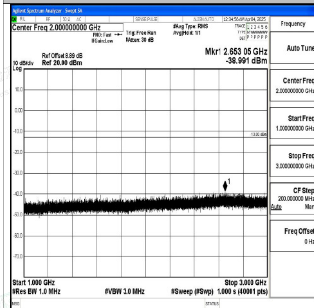
Band5_10MHz_16QAM_20450_1RB#0_1000~3000_100
