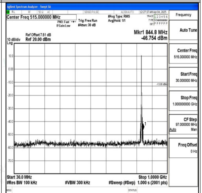
Band5_3MHz_16QAM_20525_1RB#0_30~1000_30~1000 0
