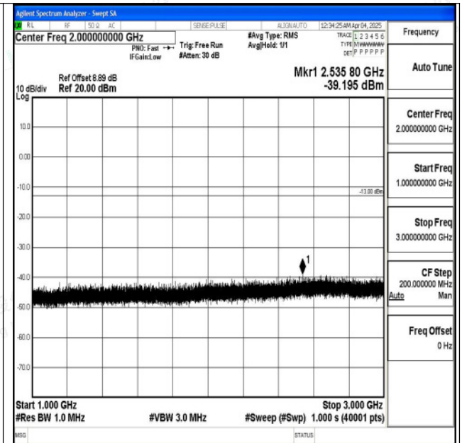
Band5_10MHz_QPSK_20450_1RB#0_1000~3000_1000 ~3000
