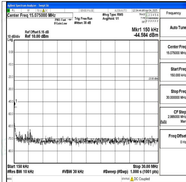
Band5_10MHz_16QAM_20450_1RB#0_0.15~30_0.15~3
