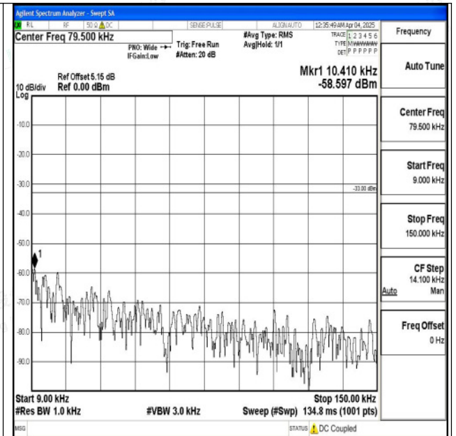
Band5_10MHz_16QAM_20525_1RB#0_0.009~0.15_0.0 09~0.15
