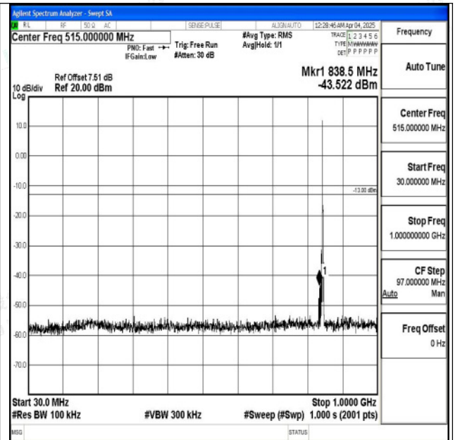
Band5_3MHz_16QAM_20635_1RB#0_30~1000_30~1000 0
