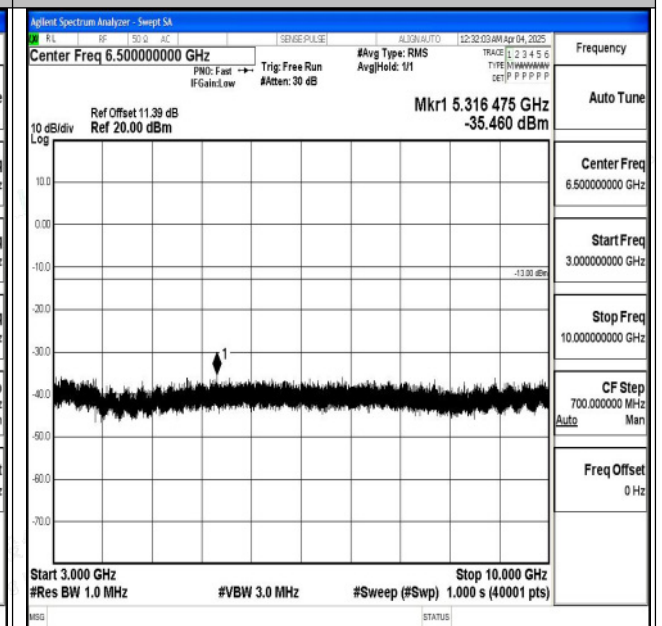
Band5_5MHz_16QAM_20525_1RB#0_3000~10000_3000~10000
