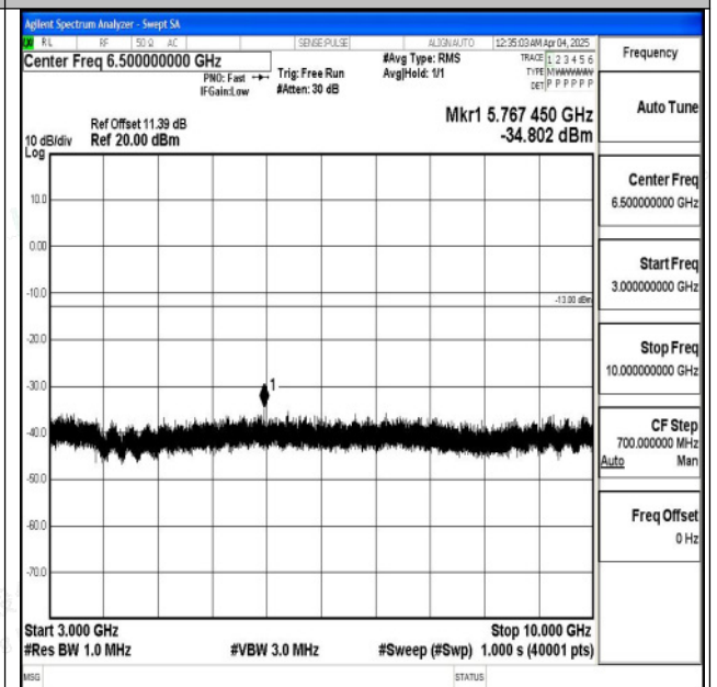
Band5_10MHz_16QAM_20450_1RB#0_3000~10000_30
