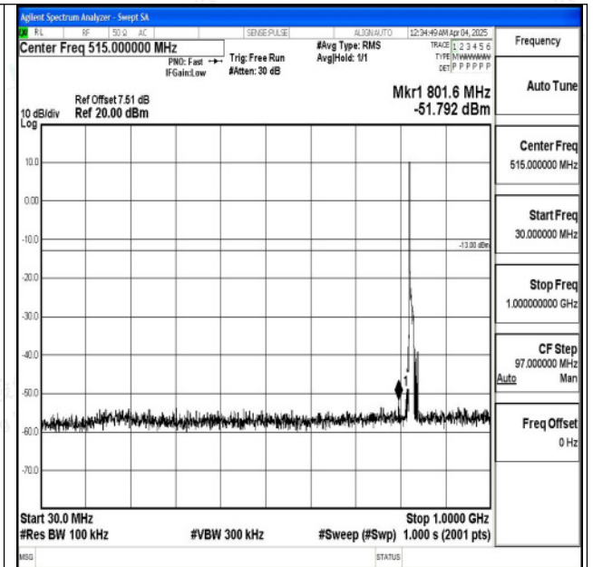
Band5_10MHz_16QAM_20450_1RB#0_30~1000_30~10
