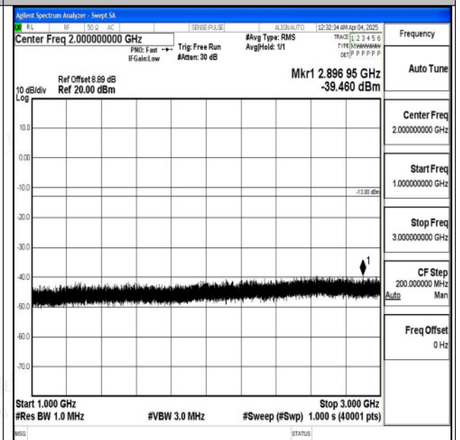
Band5_5MHz_QPSK_20625_1RB#0_1000~3000_1000~3000
