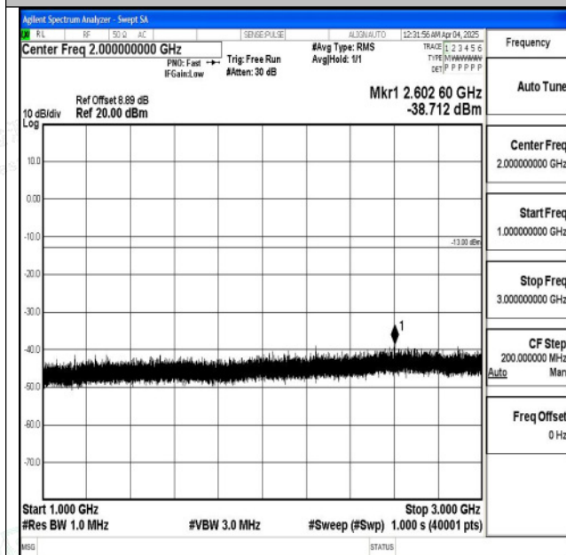
Band5_5MHz_16QAM_20525_1RB#0_1000~3000_1000~3000
