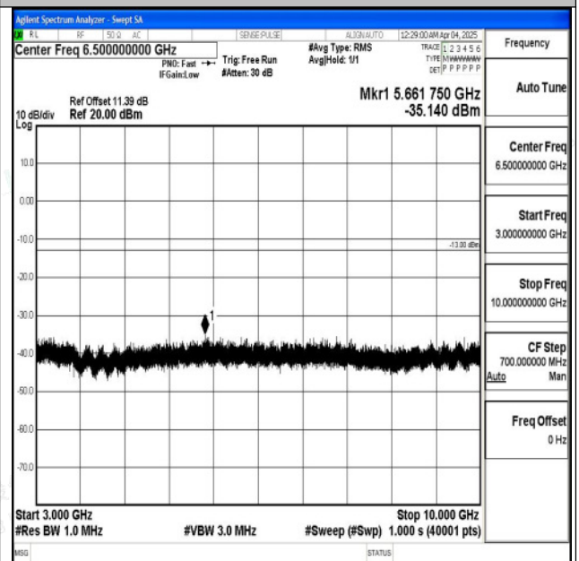
Band5_3MHz_16QAM_20635_1RB#0_3000~10000_3000 0~10000
