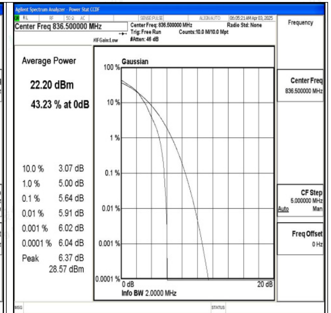
Band5-1.4MHz-16QAM-20525-1RB#0-PASS
