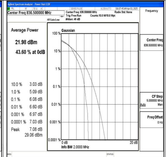
Band5-1.4MHz-16QAM-20525-6RB#0-PASS
