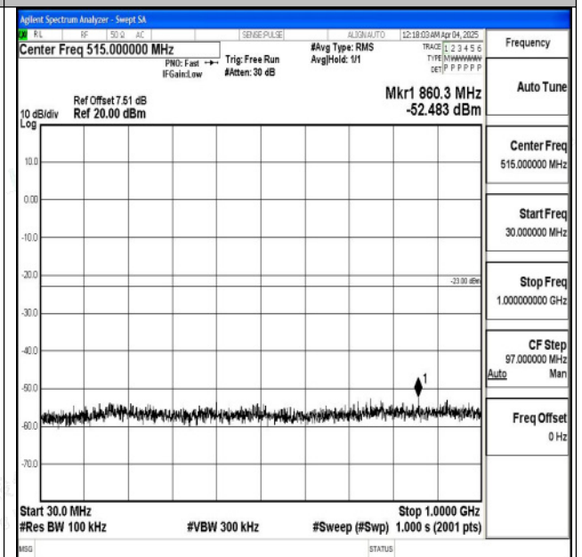
Band2_20MHz_16QAM_18900_1RB#0_30~1000_30~10 00
