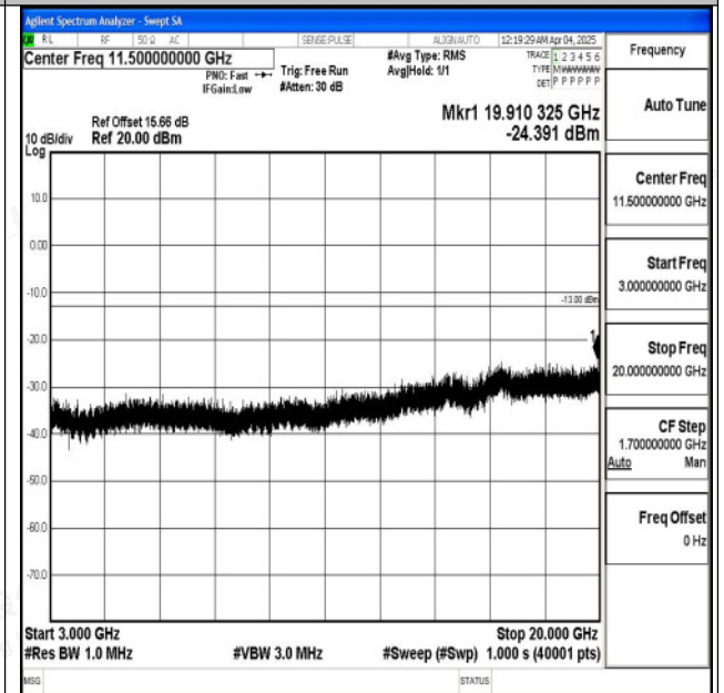
Band2_20MHz_16QAM_19100_1RB#0_3000~20000_30 00~20000
