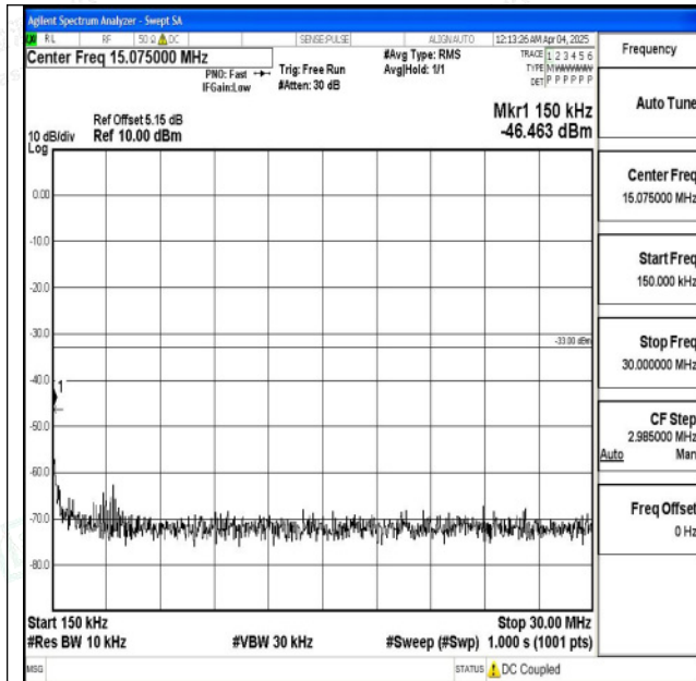
Band2_15MHz_16QAM_18900_1RB#0_0.15~30_0.15~3 0
