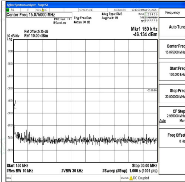
Band2_20MHz_16QAM_19100_1RB#0_0.15~30_0.15~3 0
