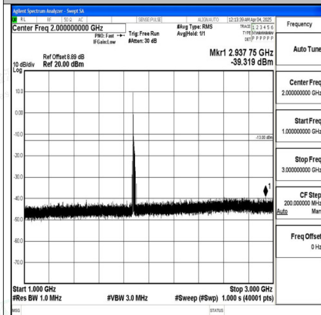
Band2_15MHz_16QAM_18900_1RB#0_1000~3000_100 0~3000
