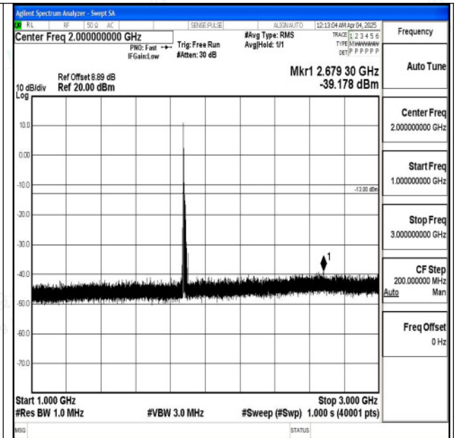
Band2_15MHz_QPSK_18900_1RB#0_1000~3000_1000 ~3000
