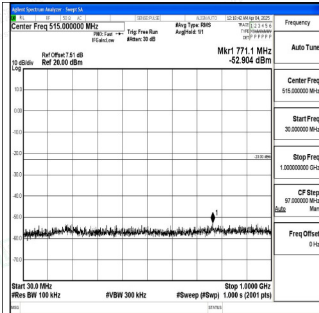
Band2_20MHz_QPSK_19100_1RB#0_30~1000_30~1000 0
