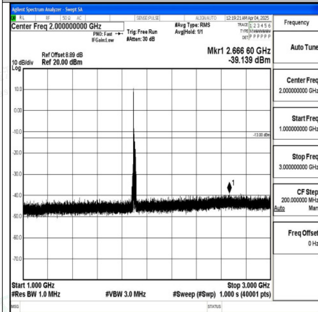
Band2_20MHz_16QAM_19100_1RB#0_1000~3000_100 0~3000
