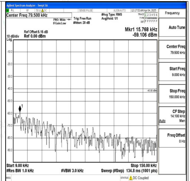
Band2_20MHz_16QAM_18900_1RB#0_0.009~0.15_0.0 09~0.15
