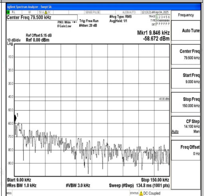
Band2_15MHz_16QAM_18900_1RB#0_0.009~0.15_0.0 09~0.15
