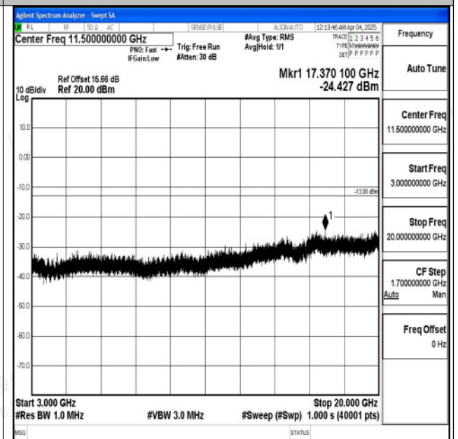
Band2_15MHz_16QAM_18900_1RB#0_3000~20000_30 00~20000
