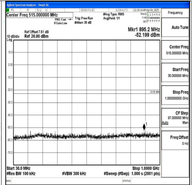
Band2_20MHz_16QAM_19100_1RB#0_30~1000_30~10 00
