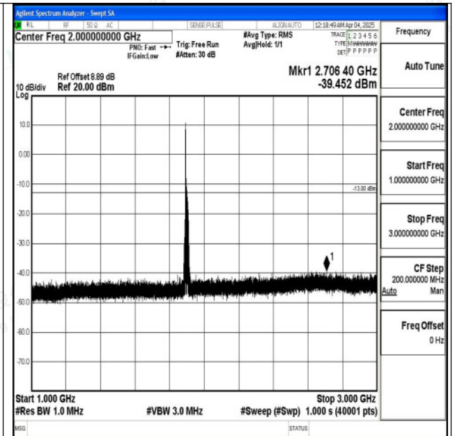
Band2_20MHz_QPSK_19100_1RB#0_1000~3000_1000 ~3000
