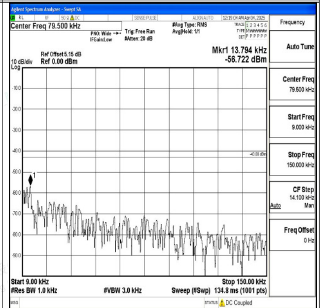
Band2_20MHz_16QAM_19100_1RB#0_0.009~0.15_0.0 09~0.15
