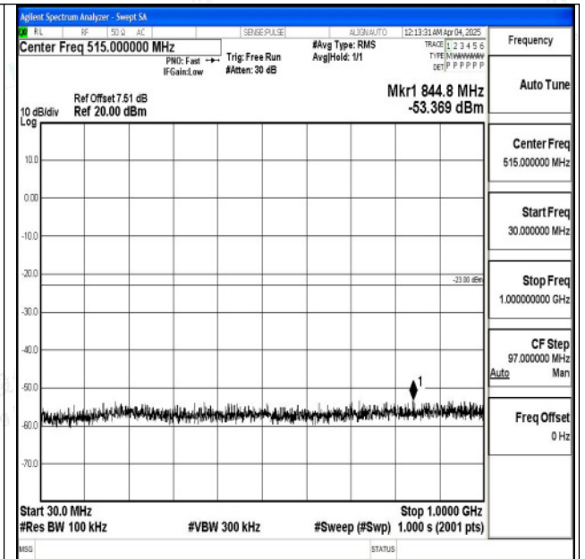
Band2_15MHz_16QAM_18900_1RB#0_30~1000_30~10 00
