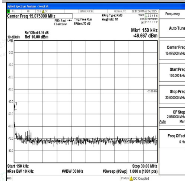
Band2_20MHz_16QAM_18900_1RB#0_0.15~30_0.15~3 0
