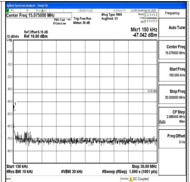
Band2_5MHz_QPSK_19175_1RB#0_0.15~30_0.15~30
