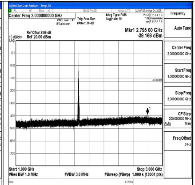
Band2_10MHz_QPSK_18650_1RB#0_1000~3000_1000 ~3000
