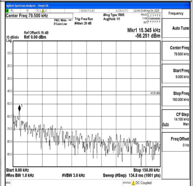
Band2_5MHz_16QAM_18900_1RB#0_0.009~0.15_0.00~0.15
