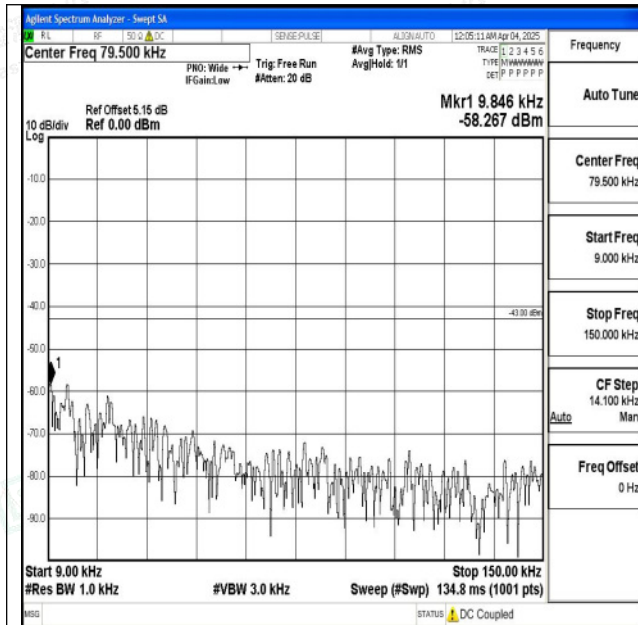
Band2_5MHz_QPSK_19175_1RB#0_0.009~0.15_0.009~0.15
