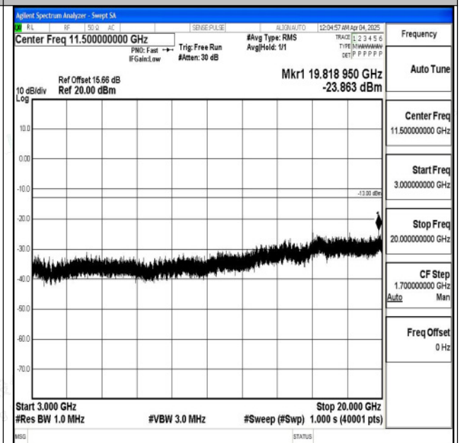
Band2_5MHz_16QAM_18900_1RB#0_3000~20000_3000 0~20000
