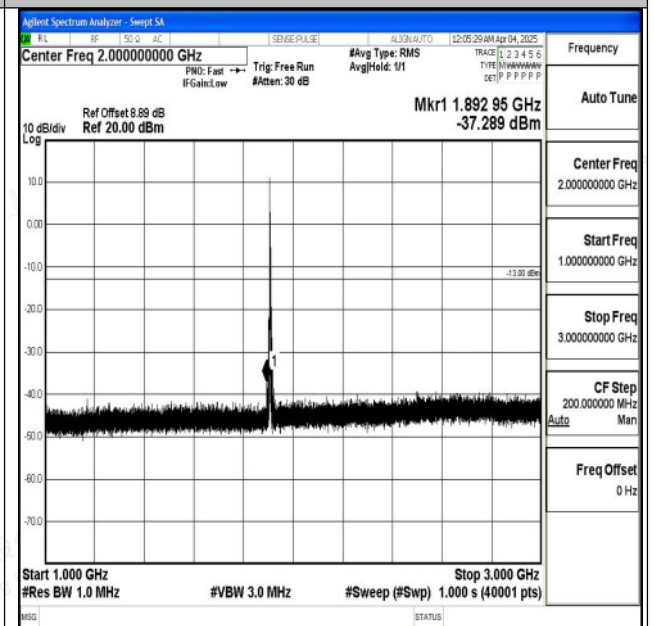
Band2_5MHz_QPSK_19175_1RB#0_1000~3000_1000~3000
