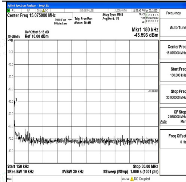
Band2_1.4MHz_16QAM_18607_1RB#0_0.15~30_0.15~ 30
