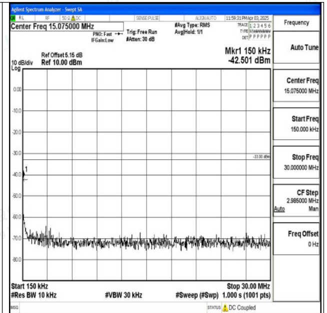
Band2_3MHz_QPSK_18900_1RB#0_0.15~30_0.15~30
