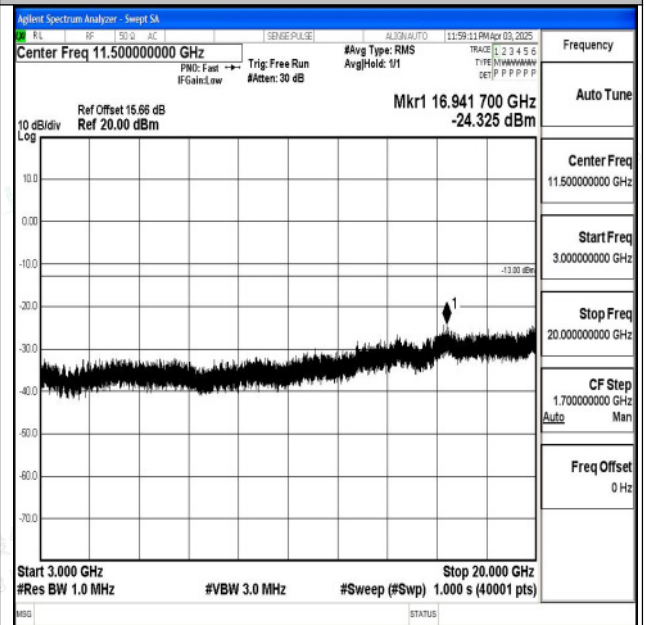
Band2_3MHz_16QAM_18615_1RB#0_3000~20000_3000 0~20000
