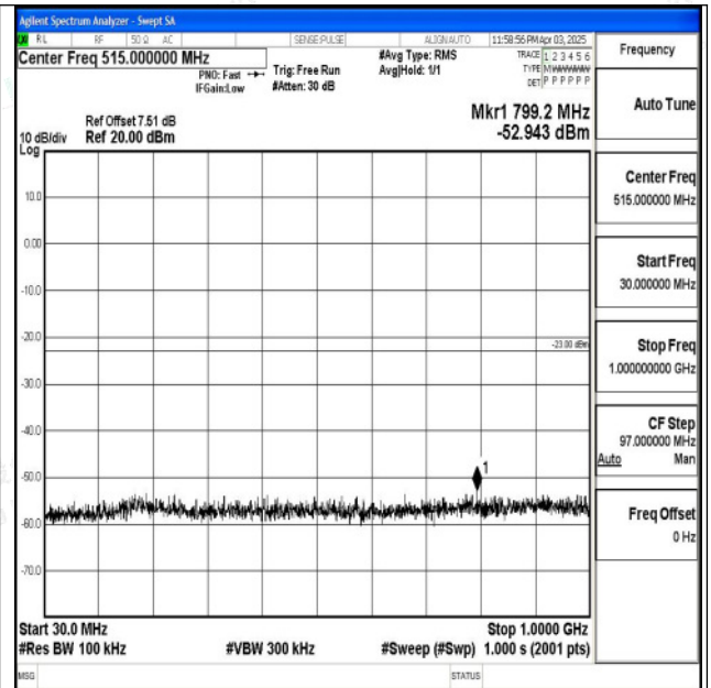
Band2_3MHz_16QAM_18615_1RB#0_30~1000_30~1000 0
