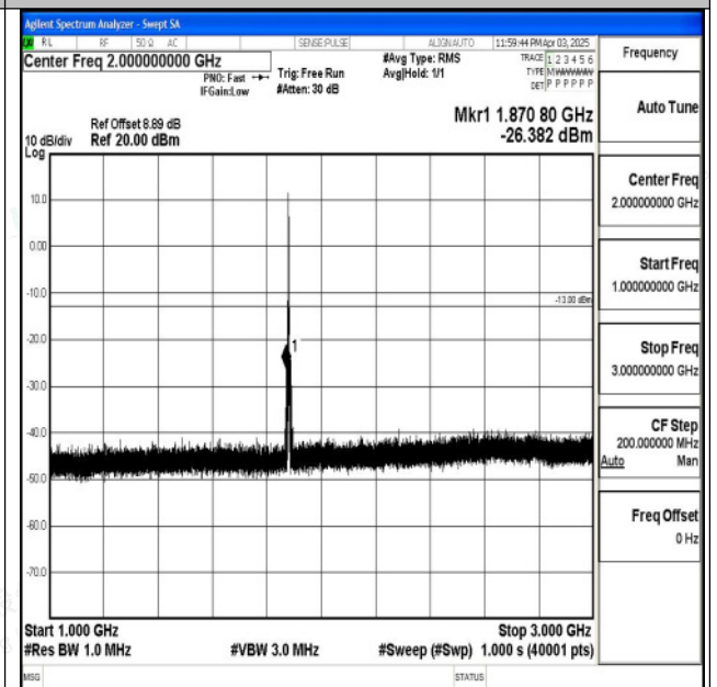
Band2_3MHz_QPSK_18900_1RB#0_1000~3000_1000~3000
