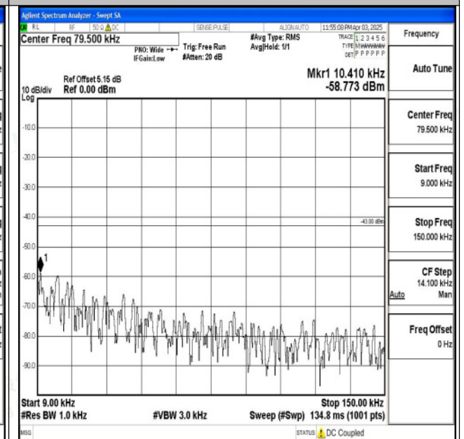
Band2_1.4MHz_16QAM_18900_1RB#0_0.009~0.15_0.0 09~0.15
