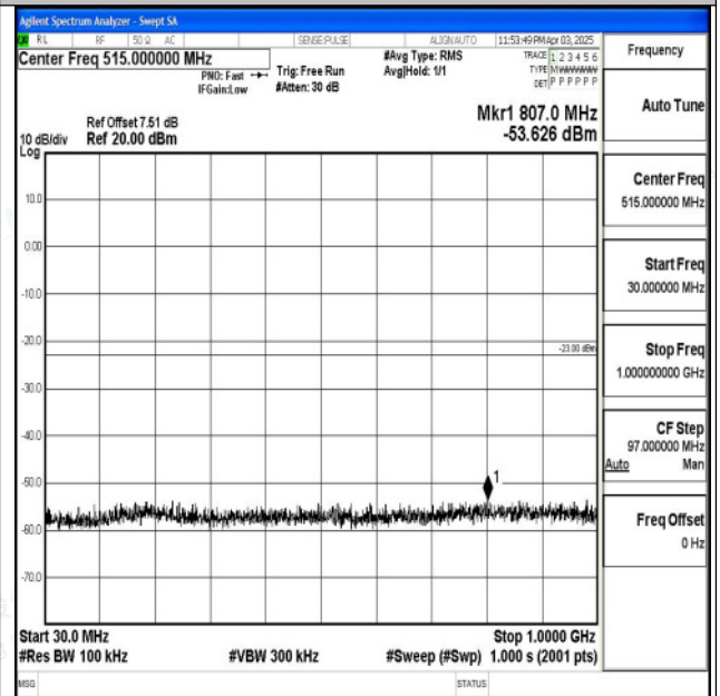
Band2_1.4MHz_16QAM_18607_1RB#0_30~1000_30~1 000
