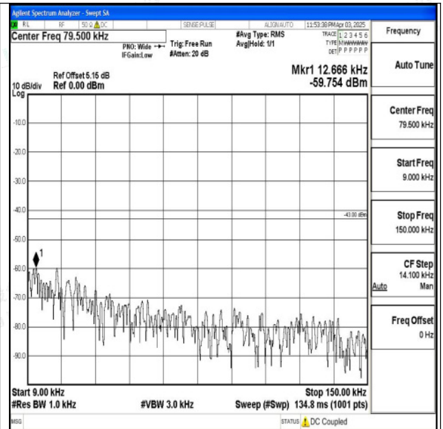
Band2_1.4MHz_16QAM_18607_1RB#0_0.009~0.15_0.0 09~0.15
