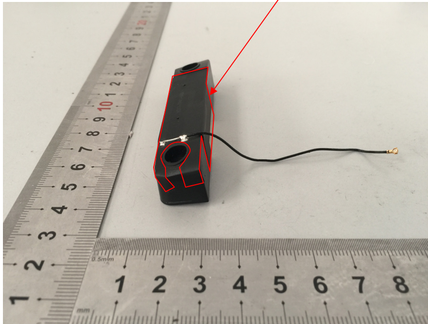
EUT – GSM/WCDMA/LTE Antenna Rear View
