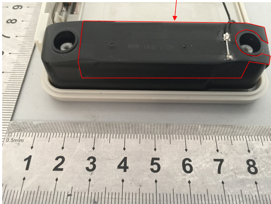
EUT – GSM/WCDMA/LTE Antenna Top View
