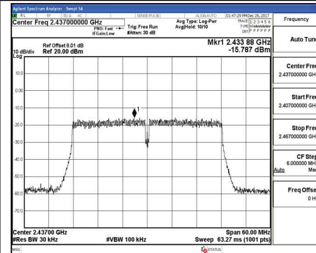
802.11n-HT40 Chain 1-Middle channel
