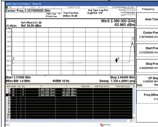
Channel 0 / 2402 MHz – Average
