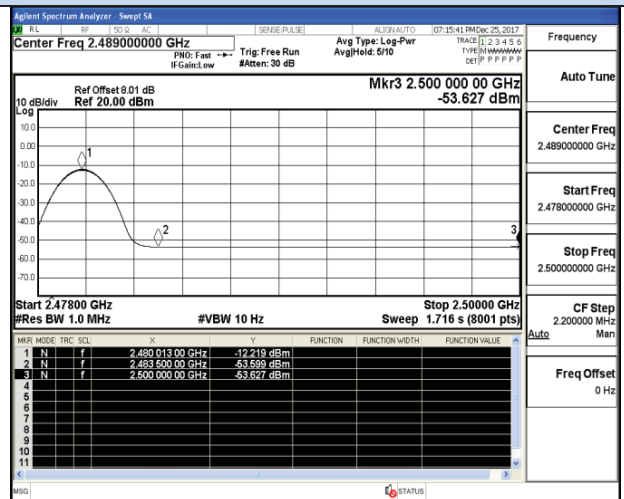
Channel 78 / 2480 MHz –Average
