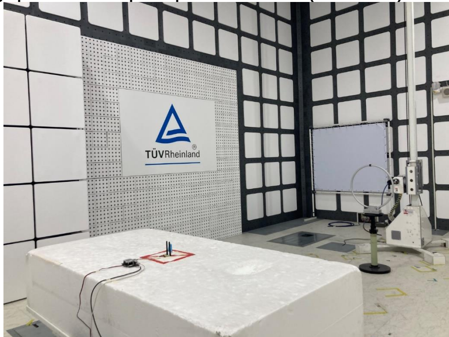
Photograph 11: Test Setup for Spurious Emissions (Back View 1)
