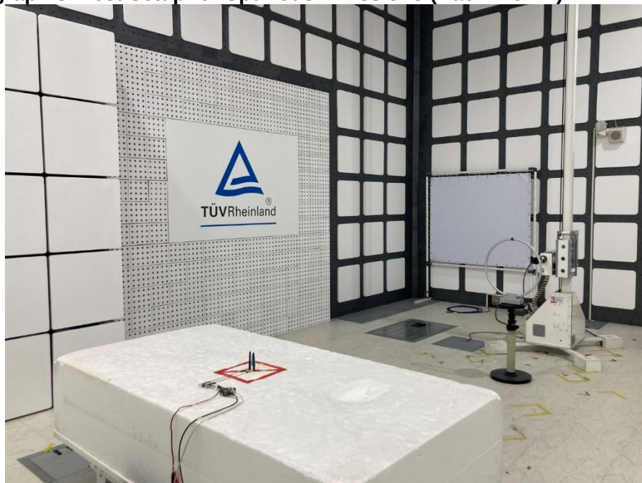
Photograph 8: Test Setup for Spurious Emissions (Back View 1)
