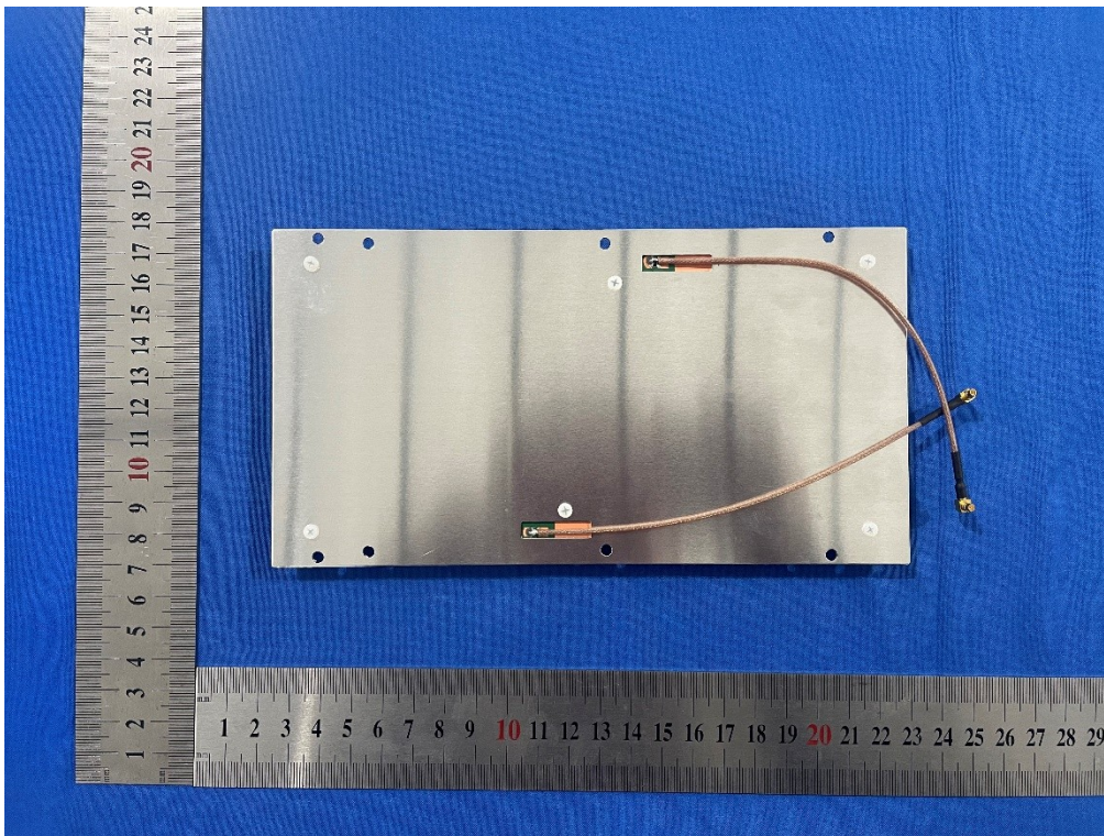
Photo 13: The product of DR5G17 Antenna view
