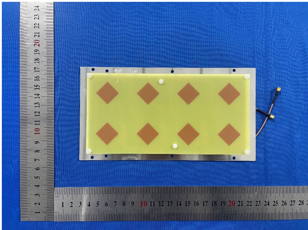
Photo 12: The product of DR5G17 Antenna view
