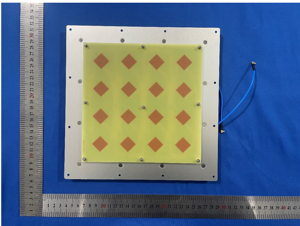
Photo 14: The product of DR5G19 Antenna view
