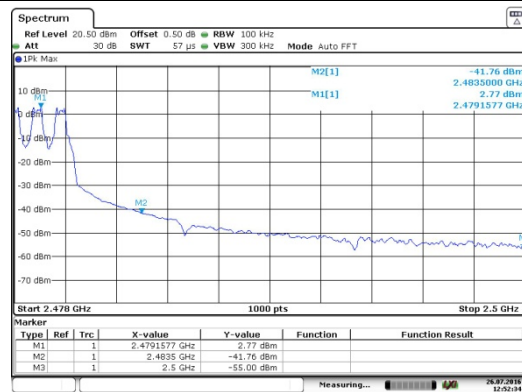
Bandedge- hopping mode (CH78)
