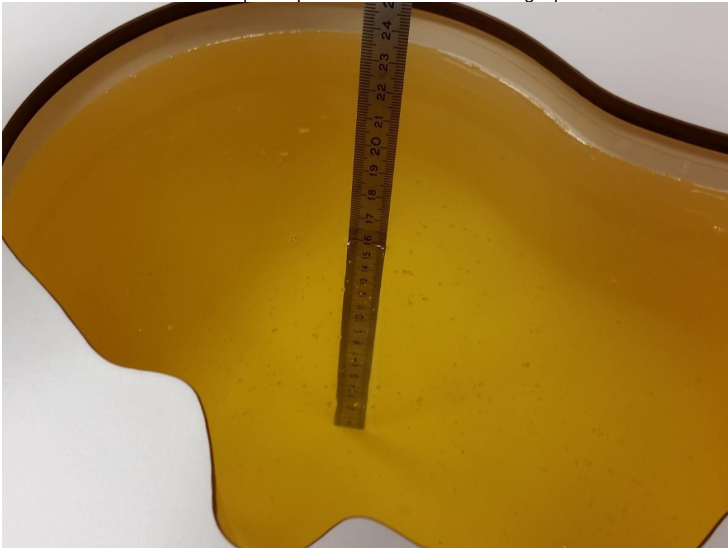
Photo 1: Liquid depth 900 MHz head simulating liquid
