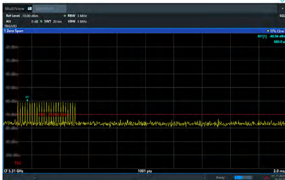
Short Pulse Radar Type 2
