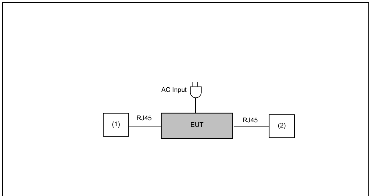
Conduction Emission
