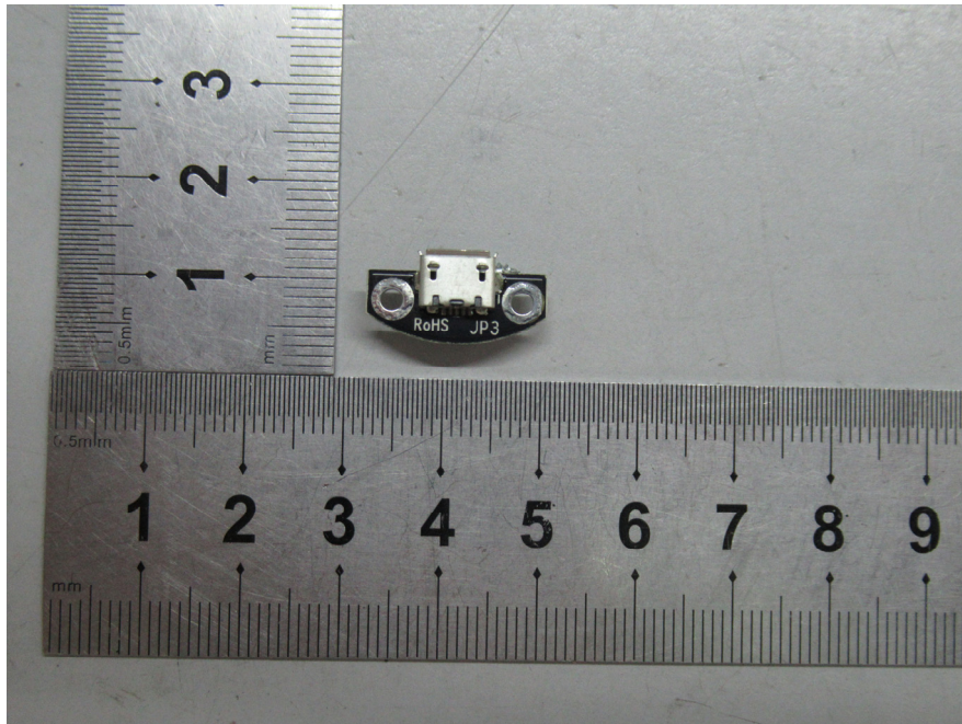
EUT (Speed 4S) – PCB3 Bottom View
