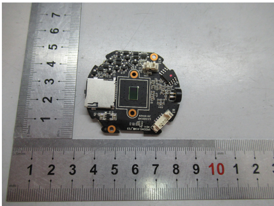
EUT (Speed 4S) – PCB1 Bottom View
