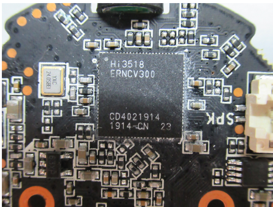
EUT (Speed 4S) – PCB1 Top Chip View-1
