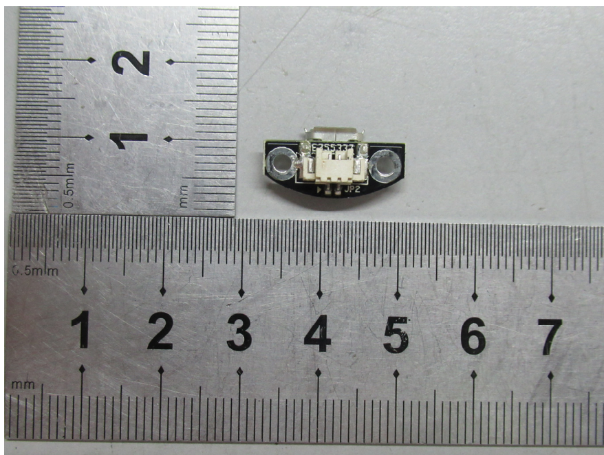
EUT (Speed 4S) – PCB3 Top View
