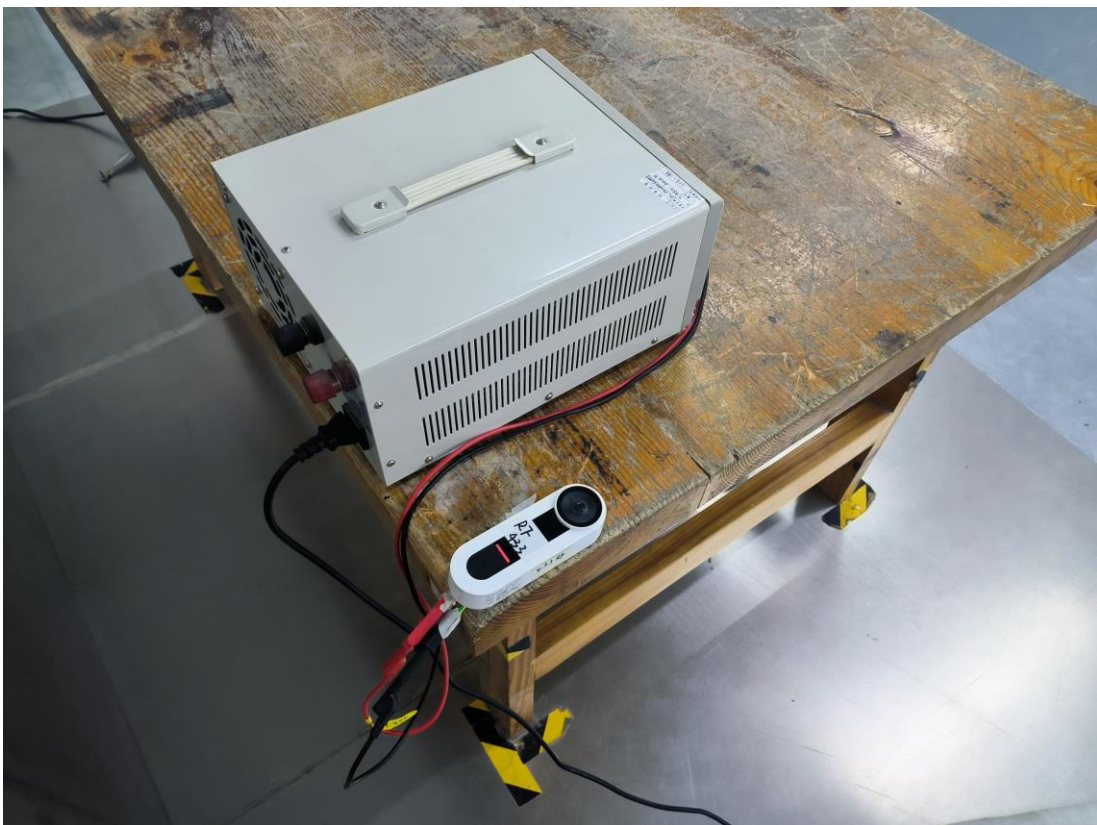
Conducted Emissions Side View DC 24V
