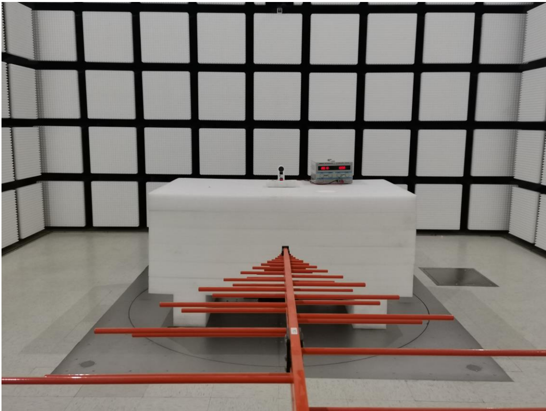
Radiated Emission Below 1GHz View (DC 24V)
