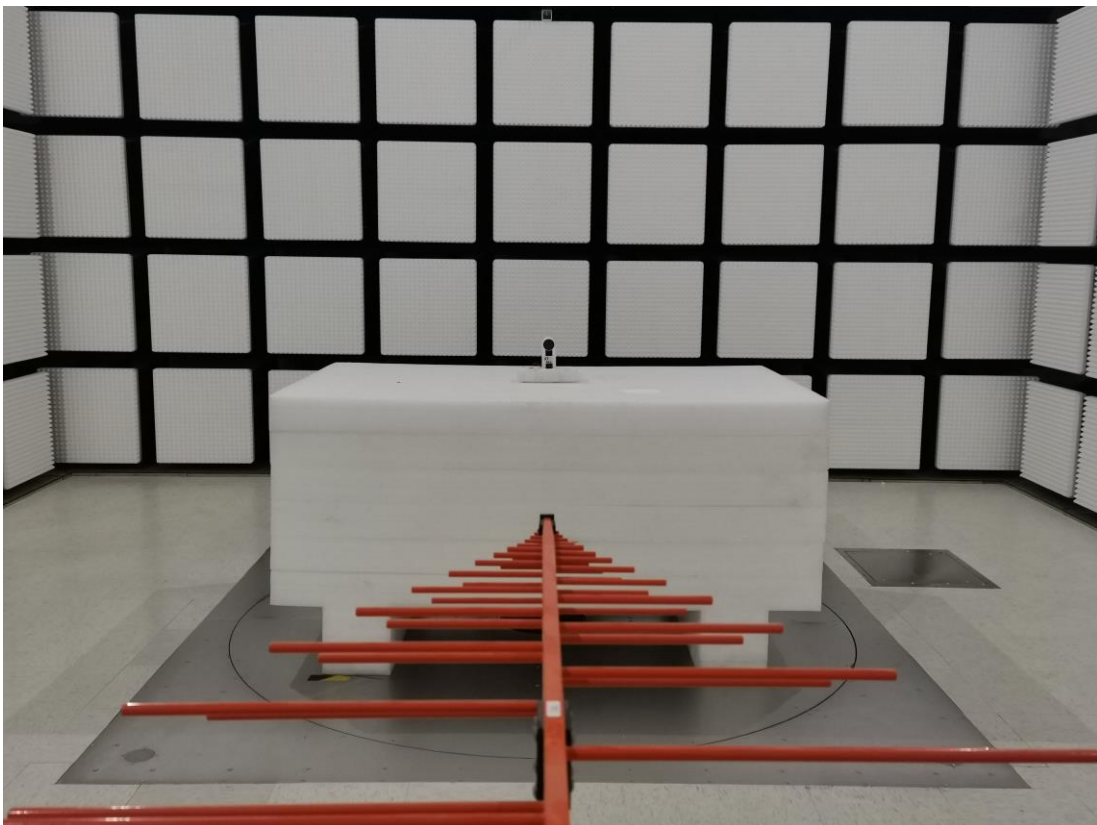
Radiated Emission Below 1GHz View (AC 12,24V)
