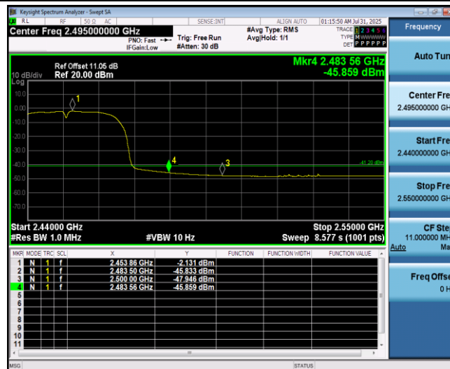
11N40SISO_Ant1_High_2452_Peak
