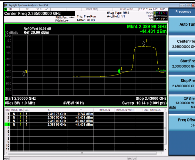
11N20SISO_Ant1_Low_2412_Peak
