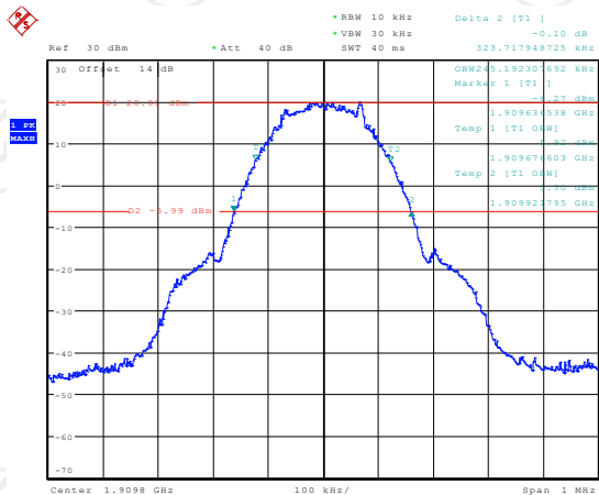
26dB&99% Occupied Bandwidth Plot on Channel 810
