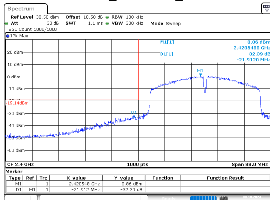
802.11n40_2422MHz_Chain 0
