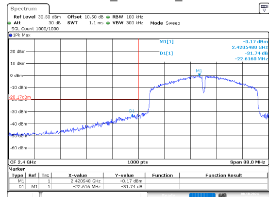
802.11n40_2422MHz_Chain 1
