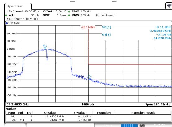
802.11n40_2452MHz_Chain 1
