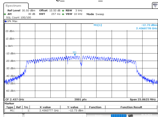
802.11g_2437MHz_Chain 1
