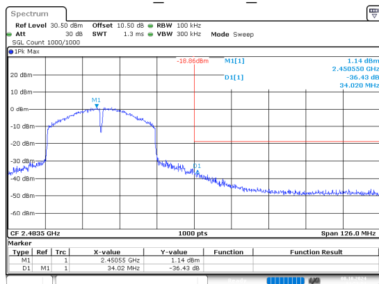
802.11n40_2452MHz_Chain 0
