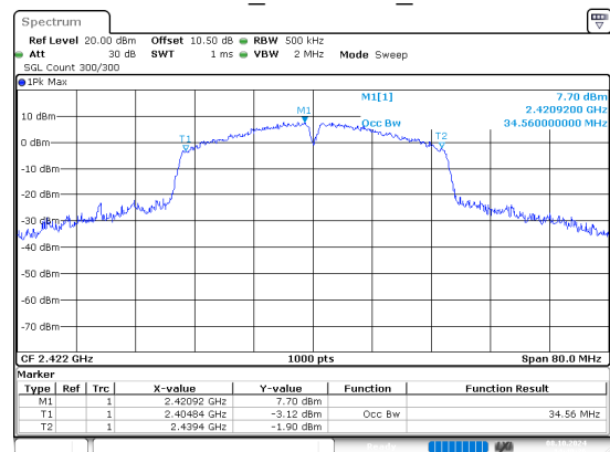
802.11n40_2422MHz_Chain 0
