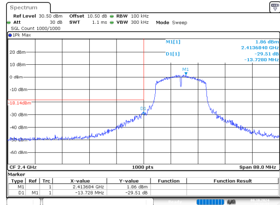
802.11g_2412MHz_Chain 1
