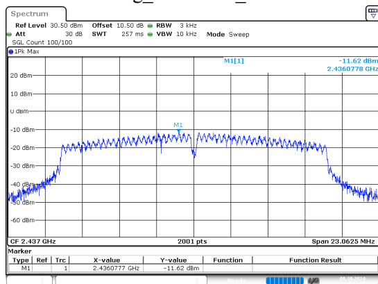
802.11g_2437MHz_Chain 0
