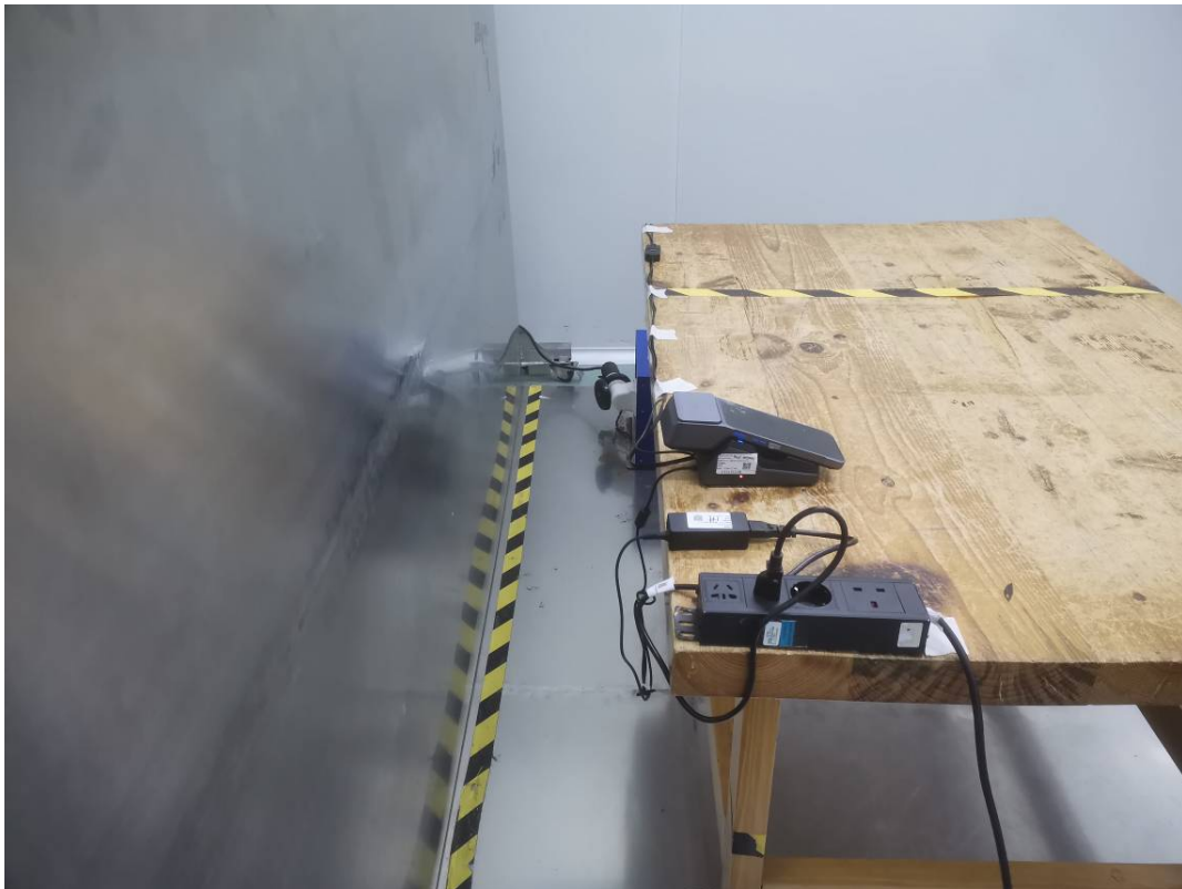
Conducted Emissions Side View Test Mode 1&3
