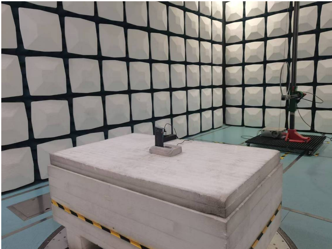
Radiated Emission 9k-30MHz Perpendicular View M1-M3
