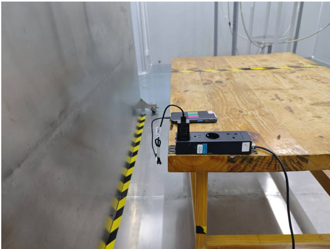
Conducted Emissions Side View M1-M3
