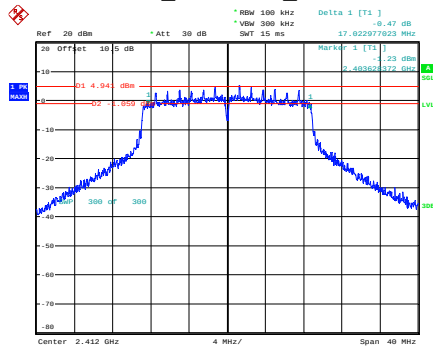
n20_2412MHz_Chain 0
