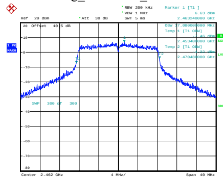
g_2462MHz_Chain 0
