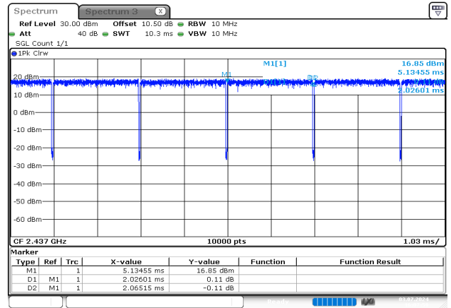
g_2437MHz_Chain 0
