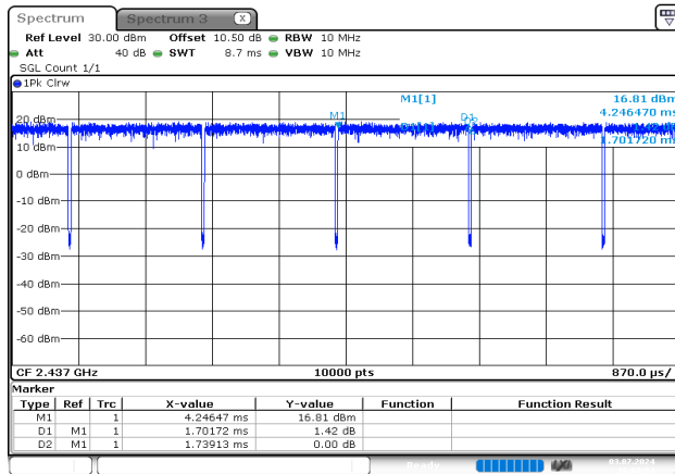
n20_2437MHz_Chain 0
