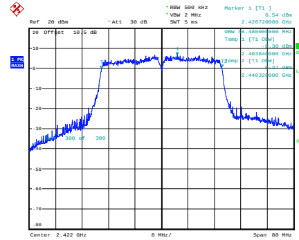
n40_2422MHz_Chain 0
