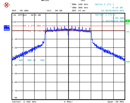
g_2462MHz_Chain 0
