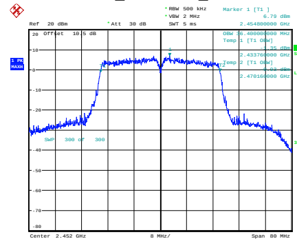
n40_2452MHz_Chain 0
