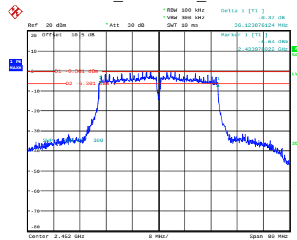
n40_2452MHz_Chain 0
