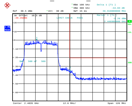
n40_2452MHz_Chain 0
