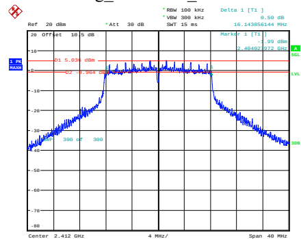
g_2412MHz_Chain 0
