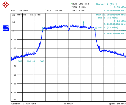
n40_2437MHz_Chain 0
