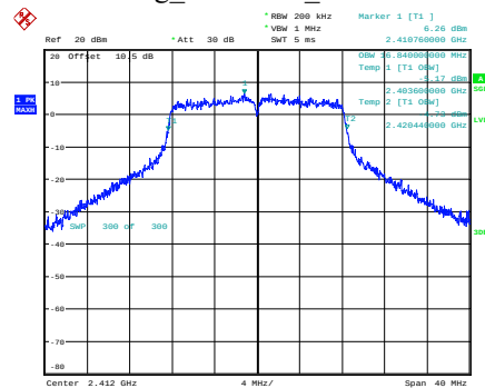
g_2412MHz_Chain 0
