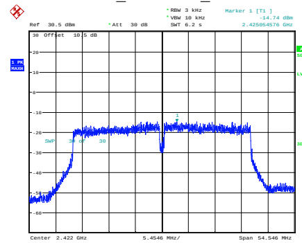
n40_2422MHz_Chain 0
