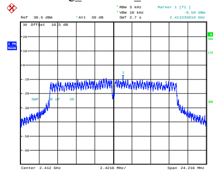
g_2412MHz_Chain 0
