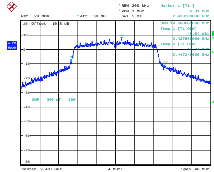
n20_2437MHz_Chain 0
