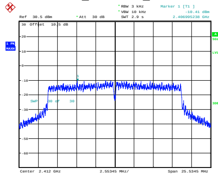
n20_2412MHz_Chain 0
