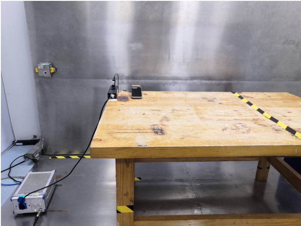
Conducted Emissions side View–Model: M20
