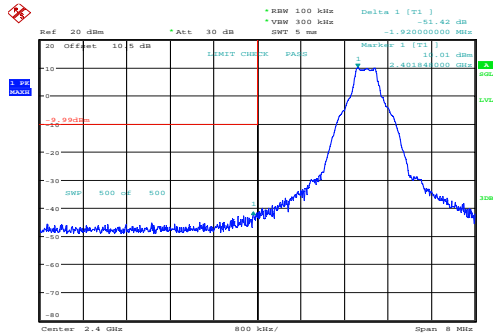
GFSK_Low
