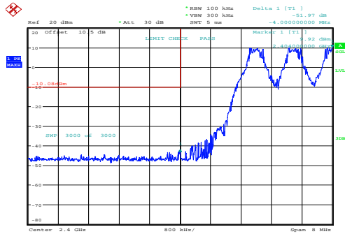
GFSK_Hopping_Lower
