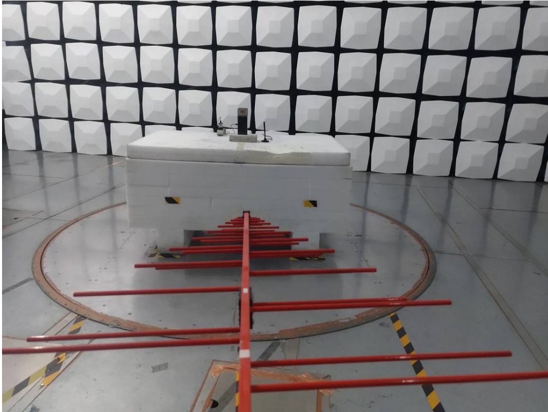
Radiated Emission Below 1G View -M20SE
