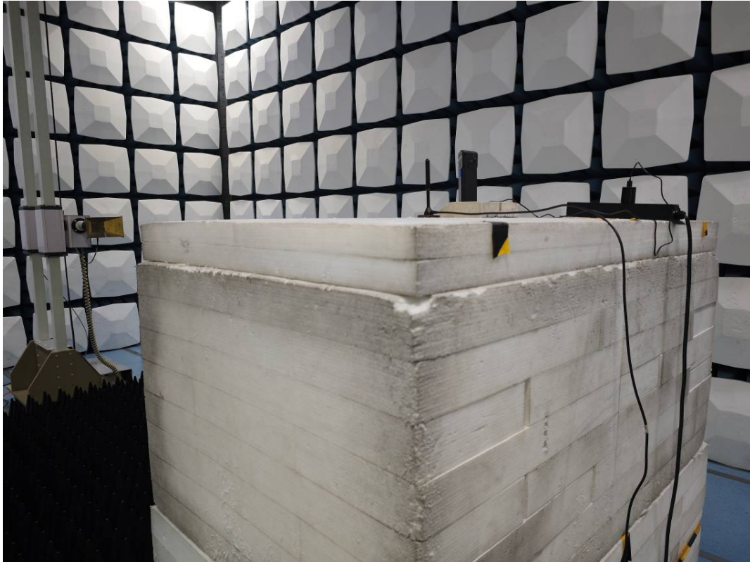
Radiated Emission 1-18GHz View-M20SE
