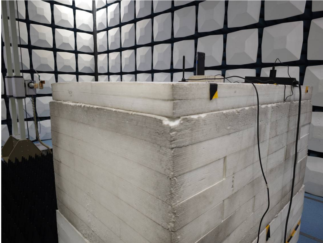
Radiated Emission 26.5-40GHz View- M20SE
