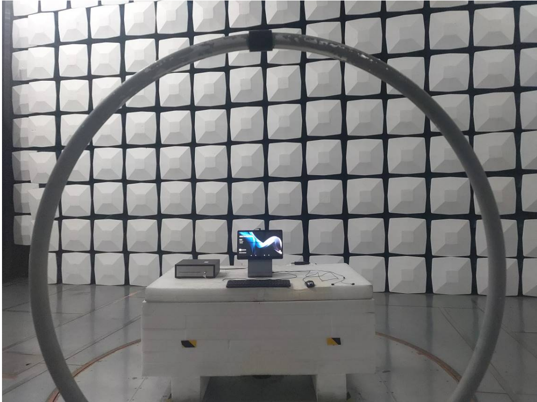
Radiated Emission 9k-30MHz Perpendicular View -Single Screen
