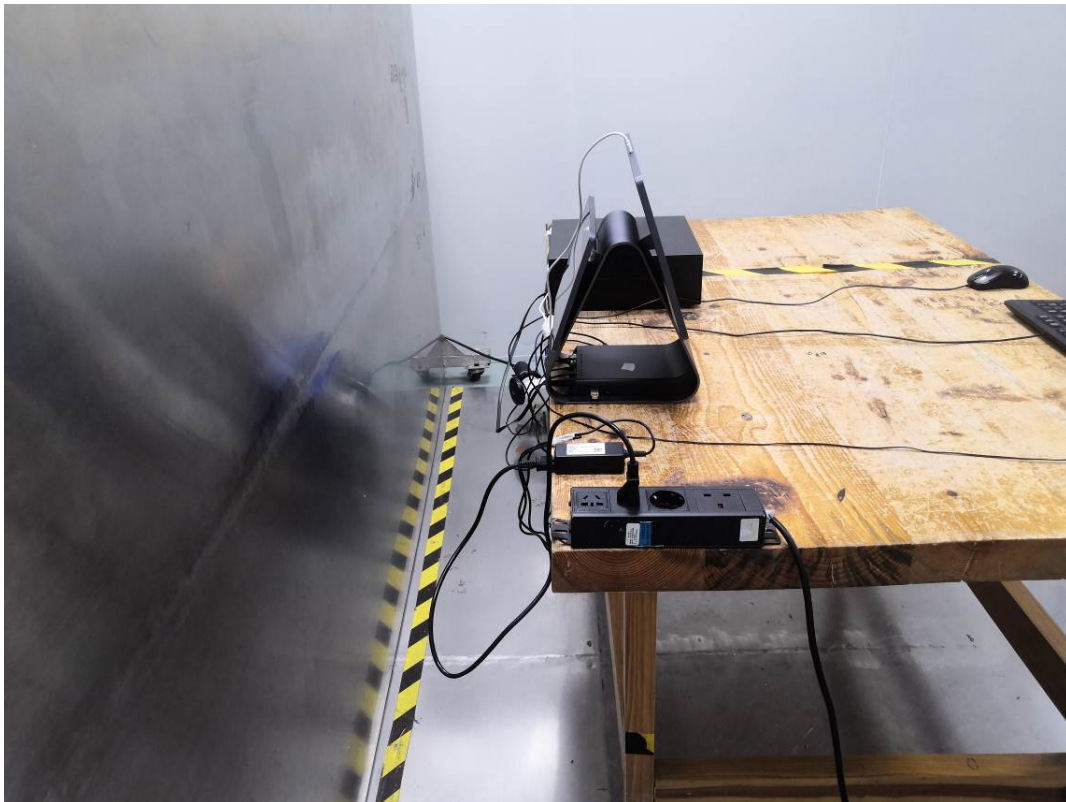
Conducted Emissions Side View-Double Screen
