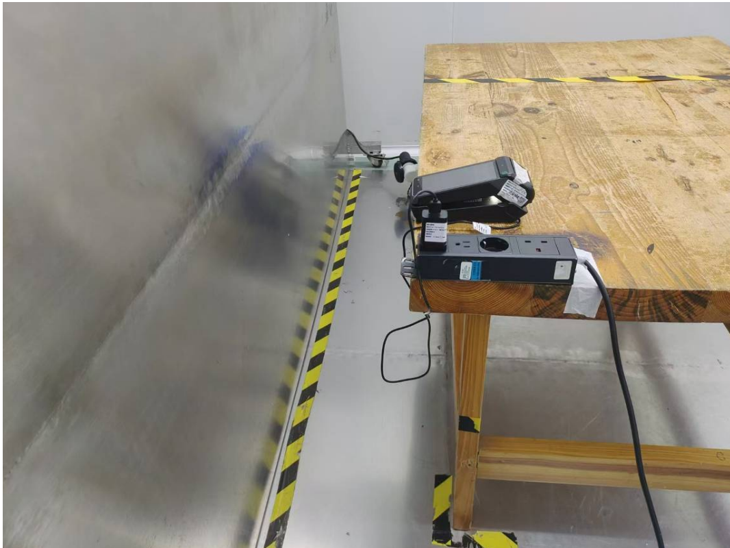
Conducted Emissions Side View-Powered by Charging Base
