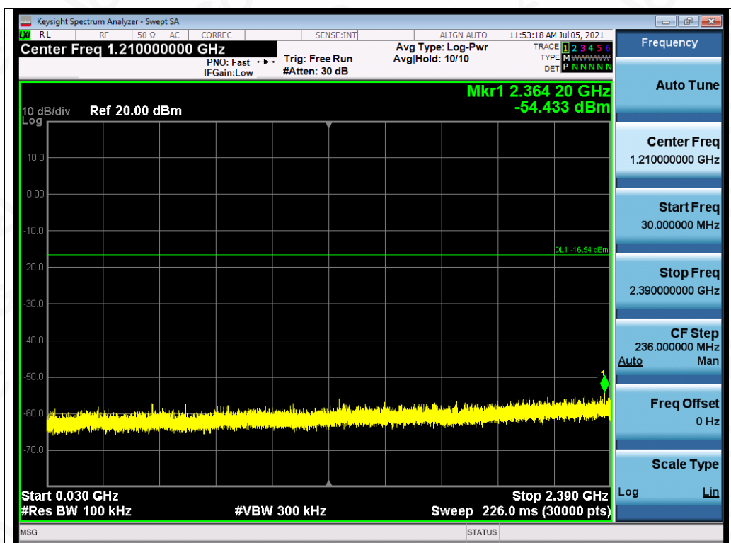
Test_Graph_OFDM_ANT1_2412_MCS0_Lower Band Emissions
