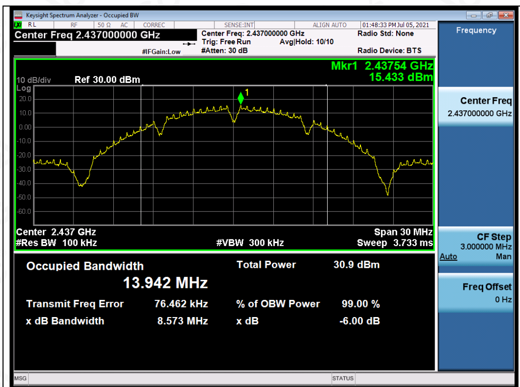
Test_Graph_802.11b_ANT2_2437_1Mbps_DTSBW
