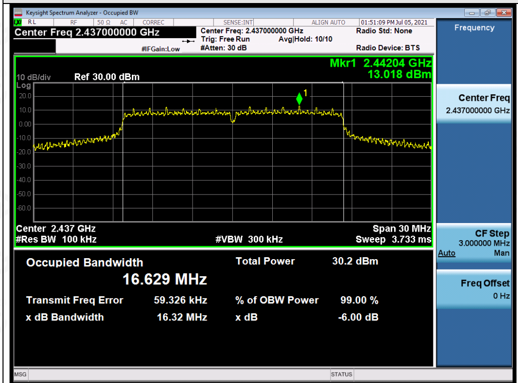
Test_Graph_802.11g_ANT2_2437_6Mbps_DTSBW
