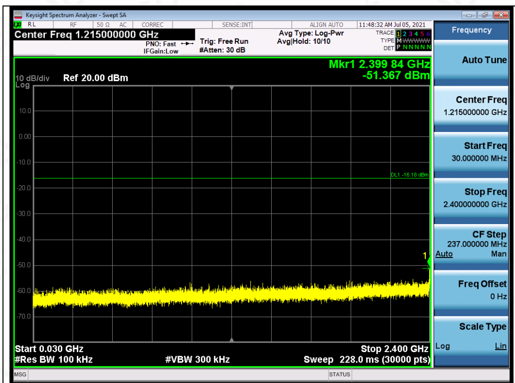
Test_Graph_OFDM_ANT1_2437_6Mbps_Lower Band Emissions
