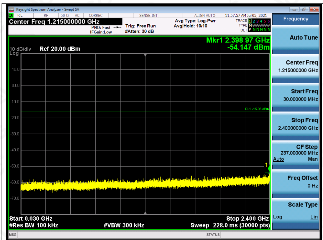
Test_Graph_OFDM_ANT1_2462_MCS0_Lower Band Emissions
