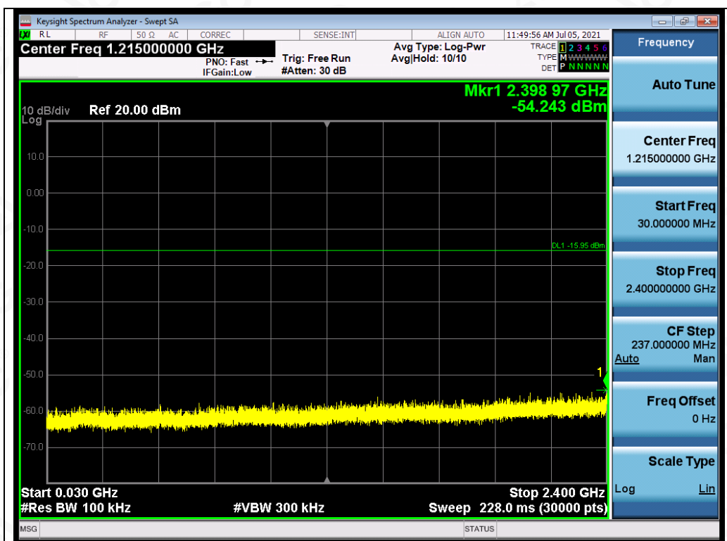
Test_Graph_OFDM_ANT1_2462_6Mbps_Lower Band Emissions
