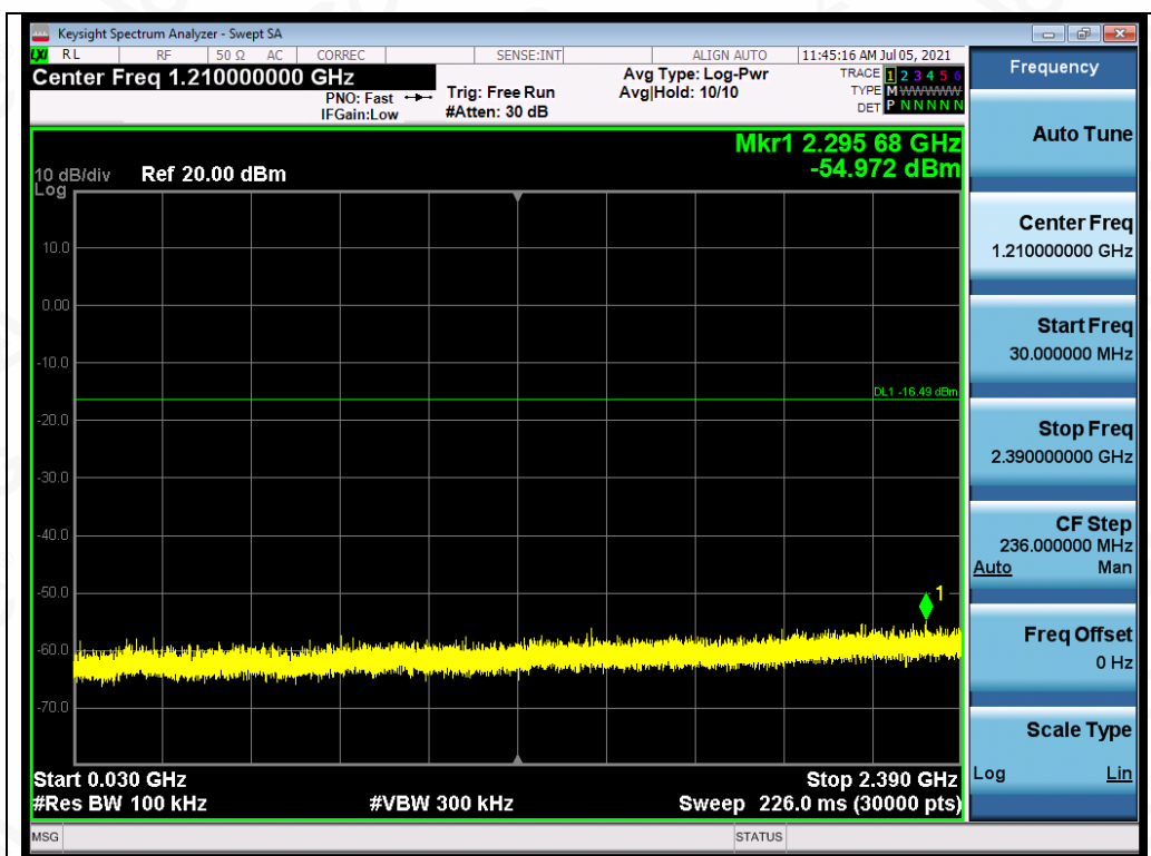
Test_Graph_OFDM_ANT1_2412_6Mbps_Lower Band Emissions
