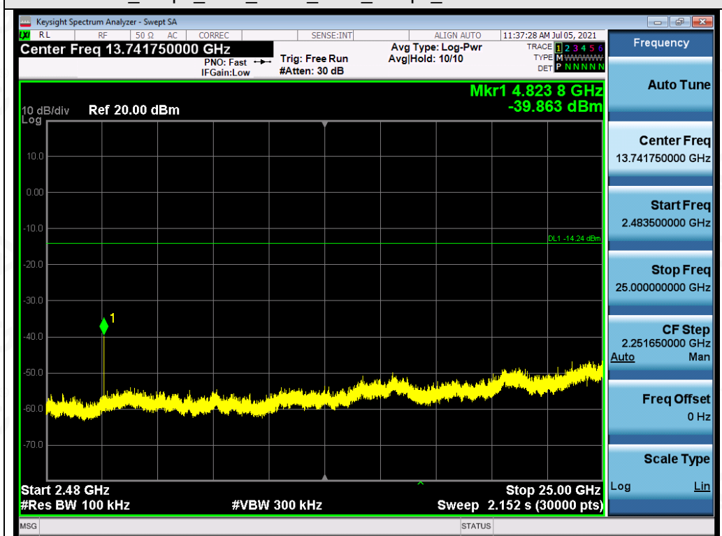
Test_Graph_CCK_ANT1_2412_1Mbps_Higher Band Emissions
