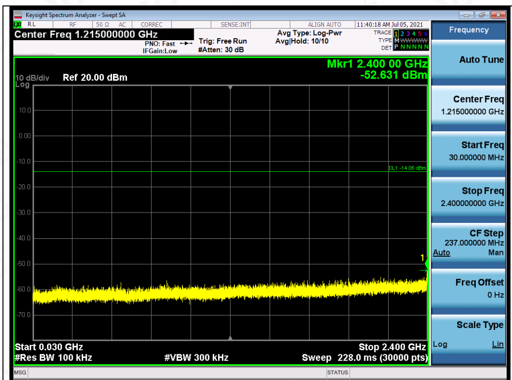
Test_Graph_CCK_ANT1_2437_1Mbps_Lower Band Emissions
