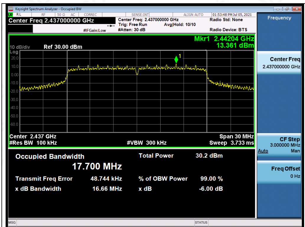
Test_Graph_802.11n20_ANT2_2437_MCS0_DTSBW
