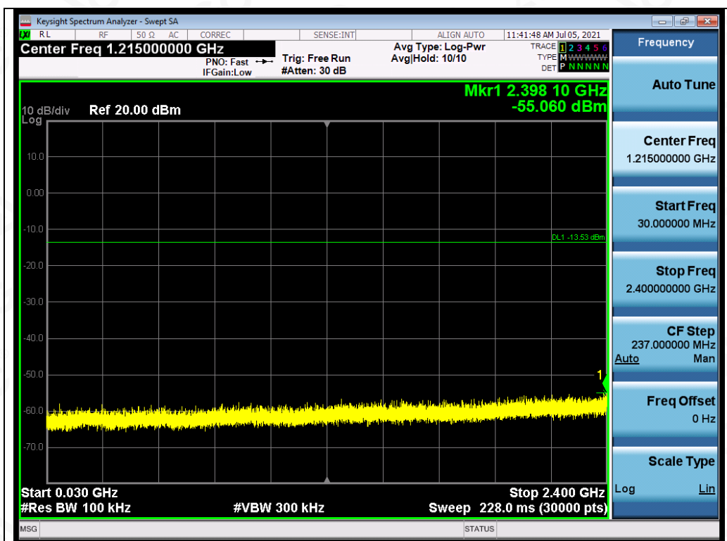
Test_Graph_CCK_ANT1_2462_1Mbps_Lower Band Emissions
