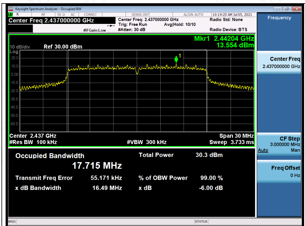
Test_Graph_802.11n20_ANT1_2437_MCS0_DTSBW
