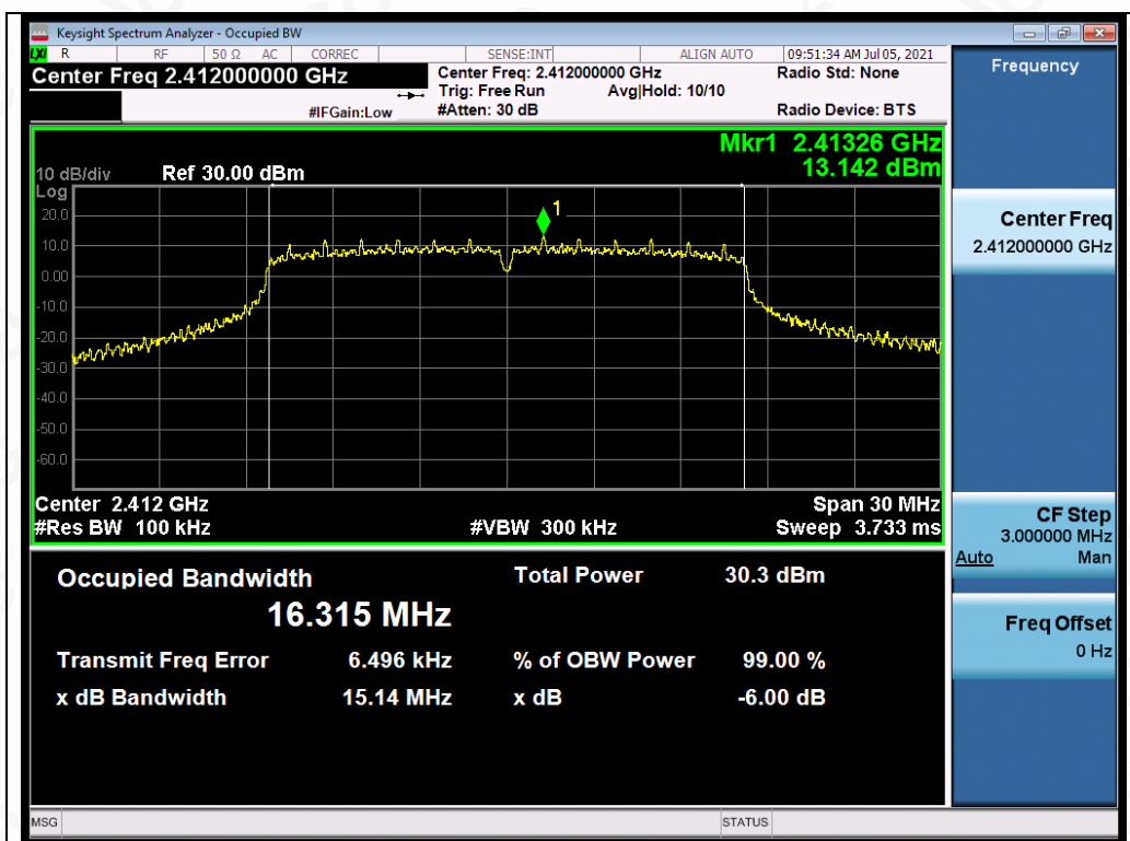
Test_Graph_802.11g_ANT1_2412_6Mbps_DTSBW
