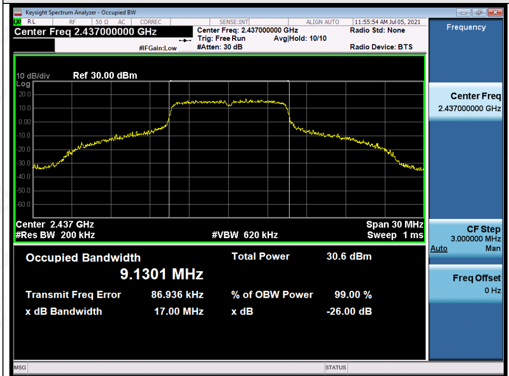
Test_Graph_OFDM_ANT1_2437_MCS0_OBW
