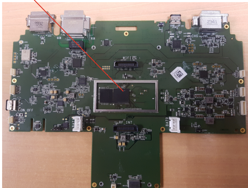
DSP and memory ( without the shielding )
