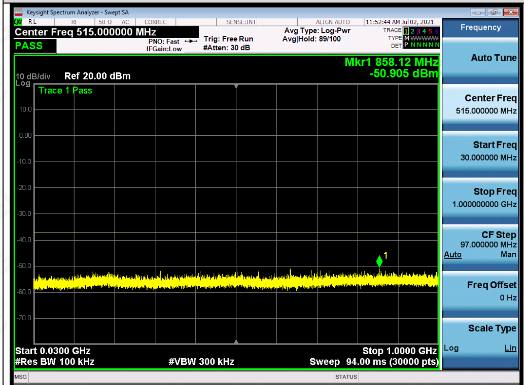
Test_Graph_OFDM_ANT1_5825_6Mbps_Frequency Band1
