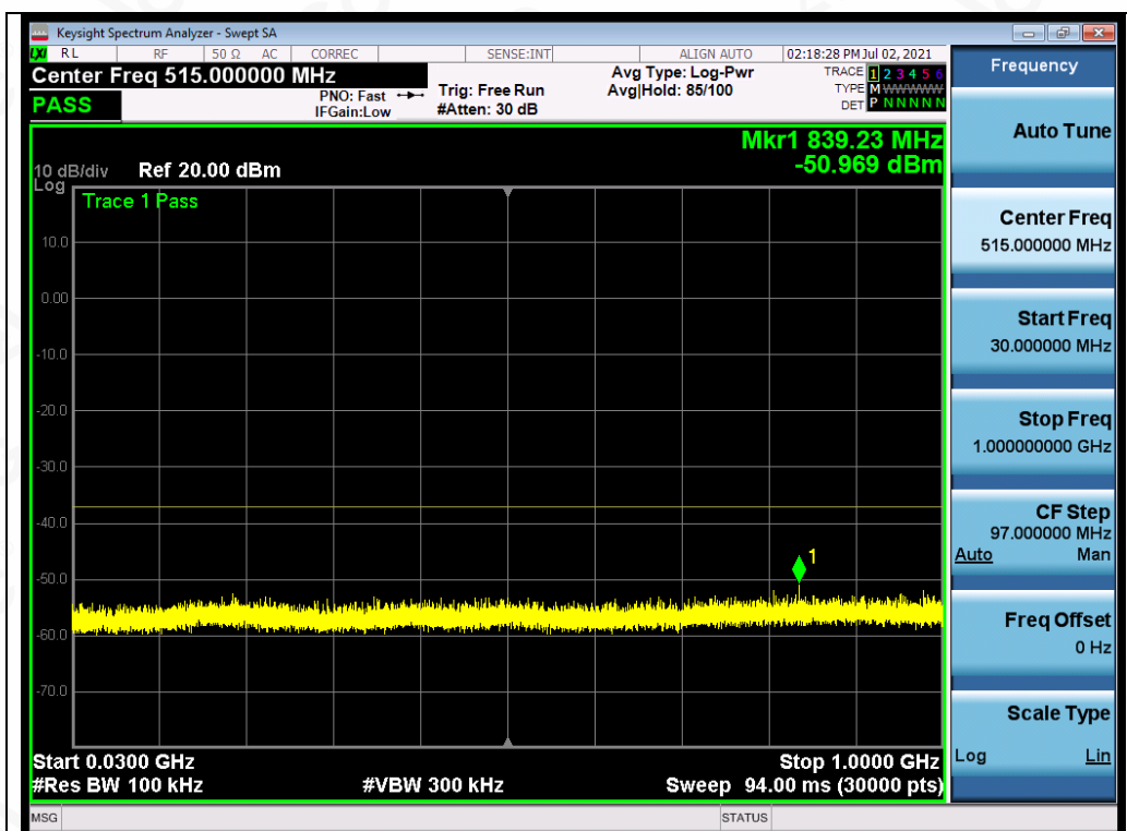
Test_Graph_802.11n20_ANT1_5745_MCS0_Frequency Band1
