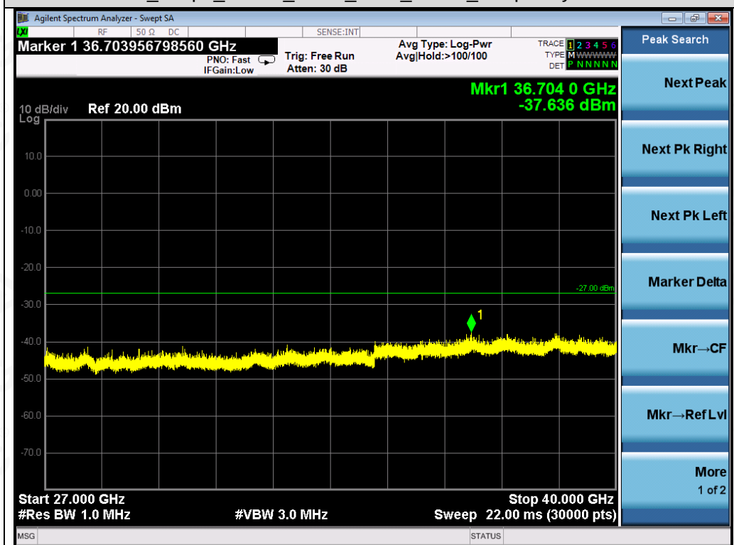
Test_Graph_OFDM_ANT1_5825_MCS0_Frequency Band5
