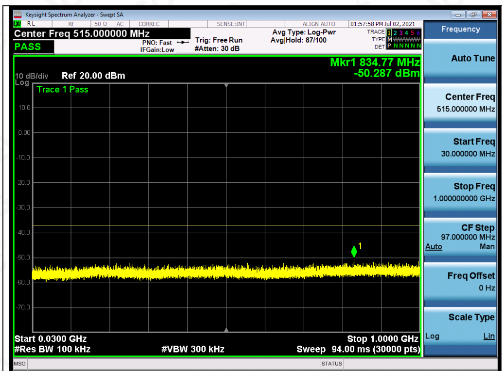
Test_Graph_OFDM_ANT1_5745_MCS0_Frequency Band1
