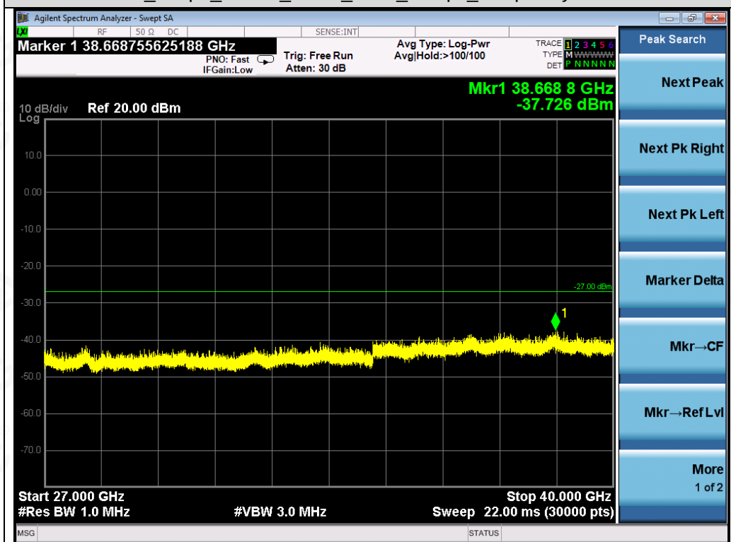
Test_Graph_OFDM_ANT1_5825_6Mbps_Frequency Band5
