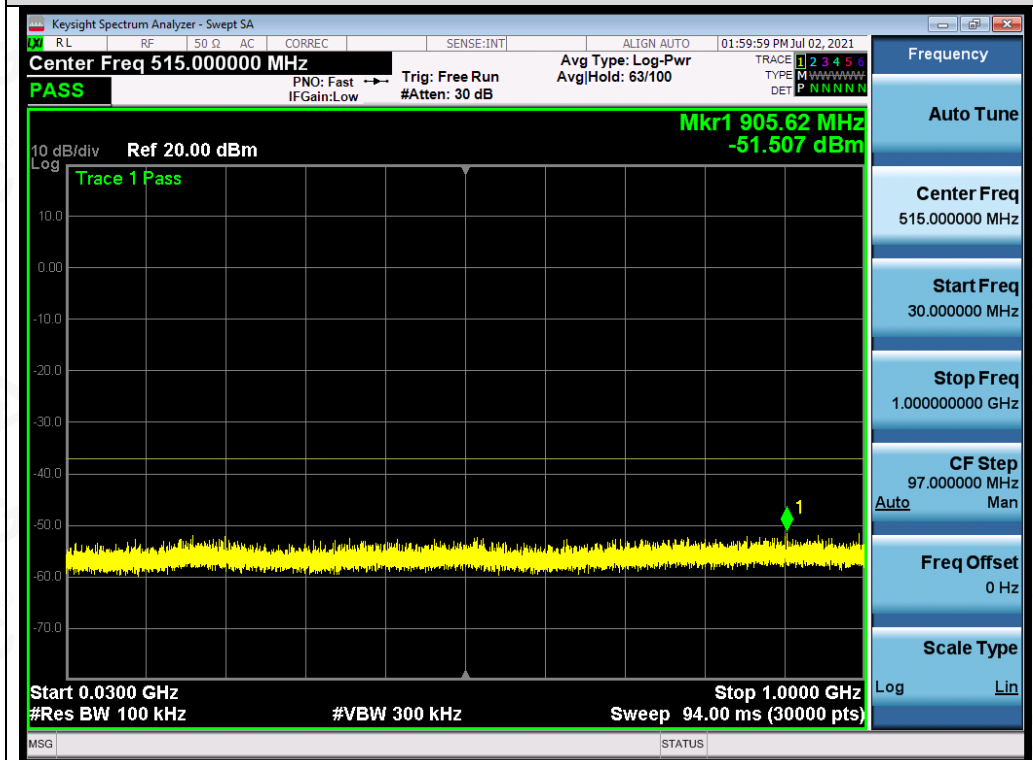
Test_Graph_OFDM_ANT1_5825_MCS0_Frequency Band1
