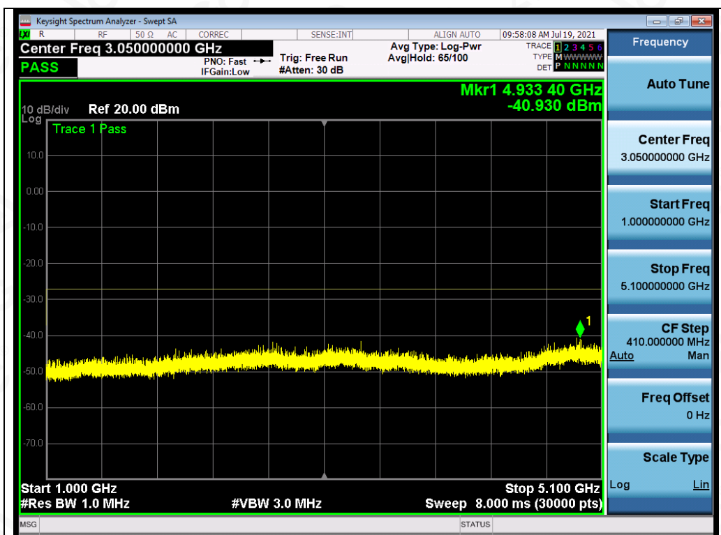
Test_Graph_OFDM_ANT1_5240_MCS0_Frequency Band 2
