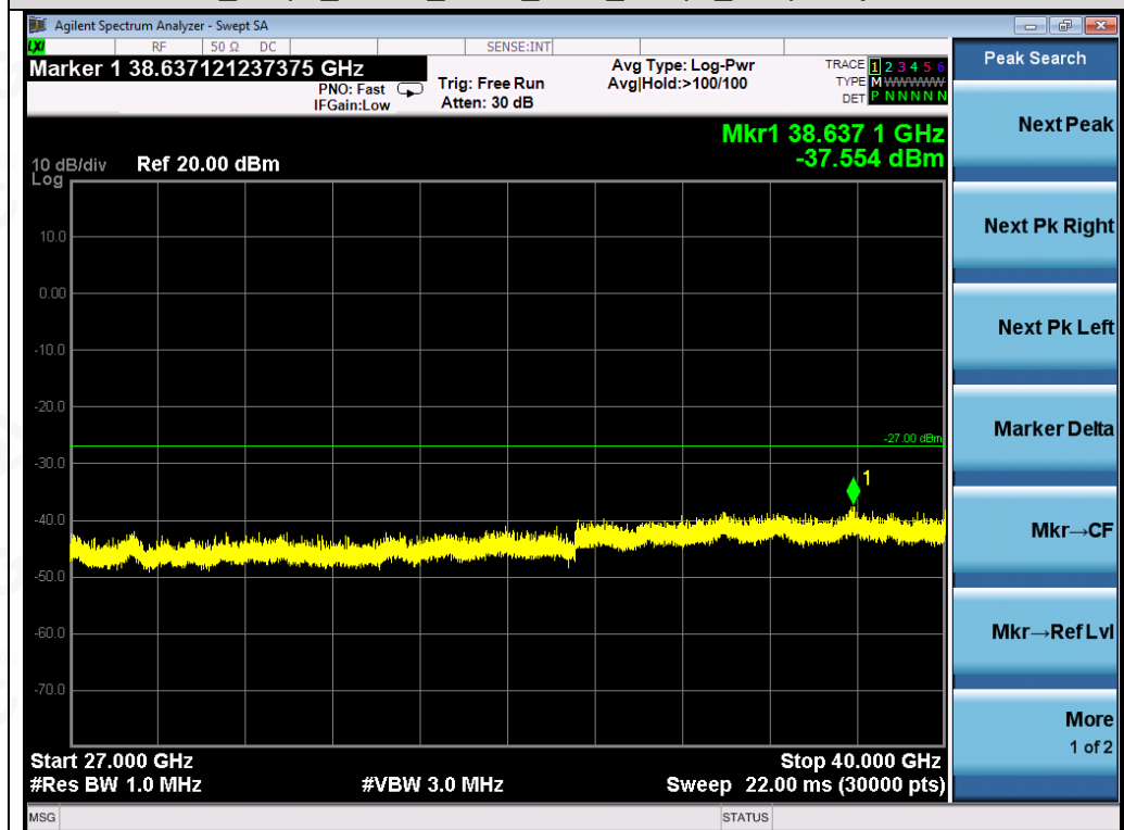
Test_Graph_OFDM_ANT1_5240_6Mbps_Frequency Band 5
