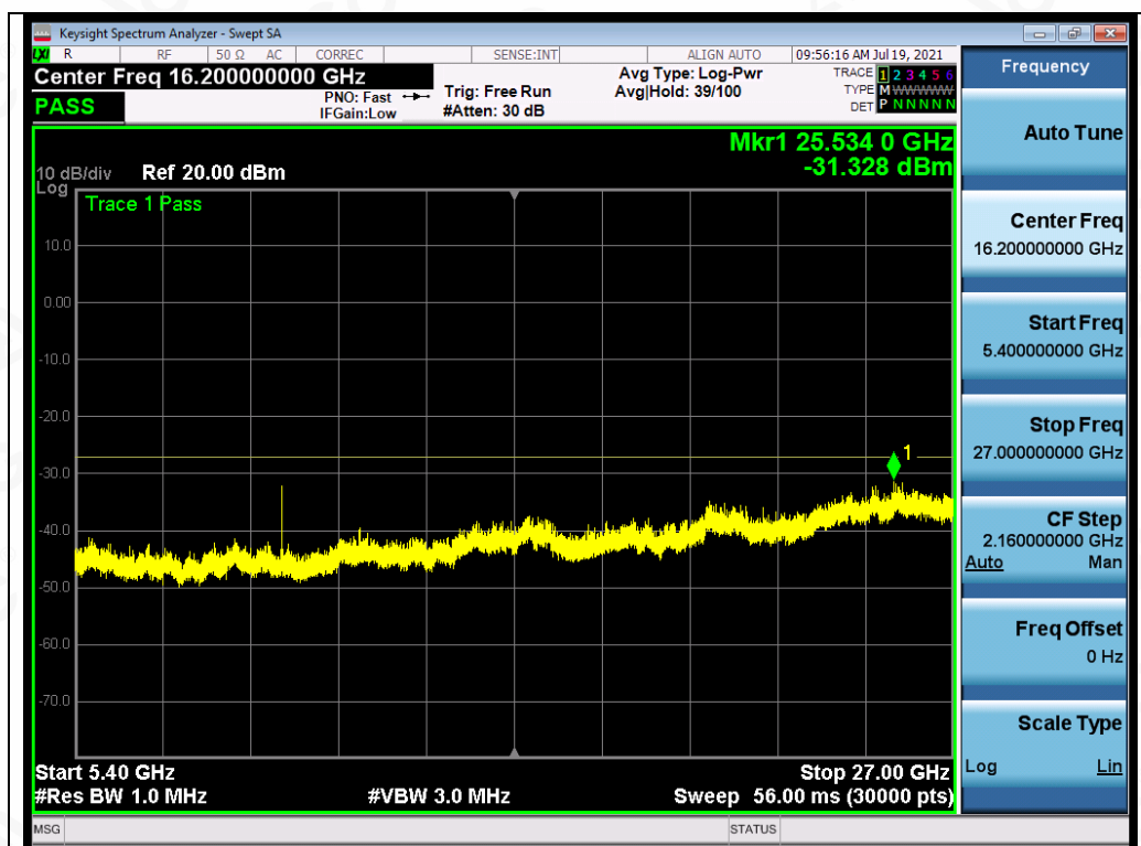
Test_Graph_OFDM_ANT1_5240_6Mbps_Frequency Band 4
