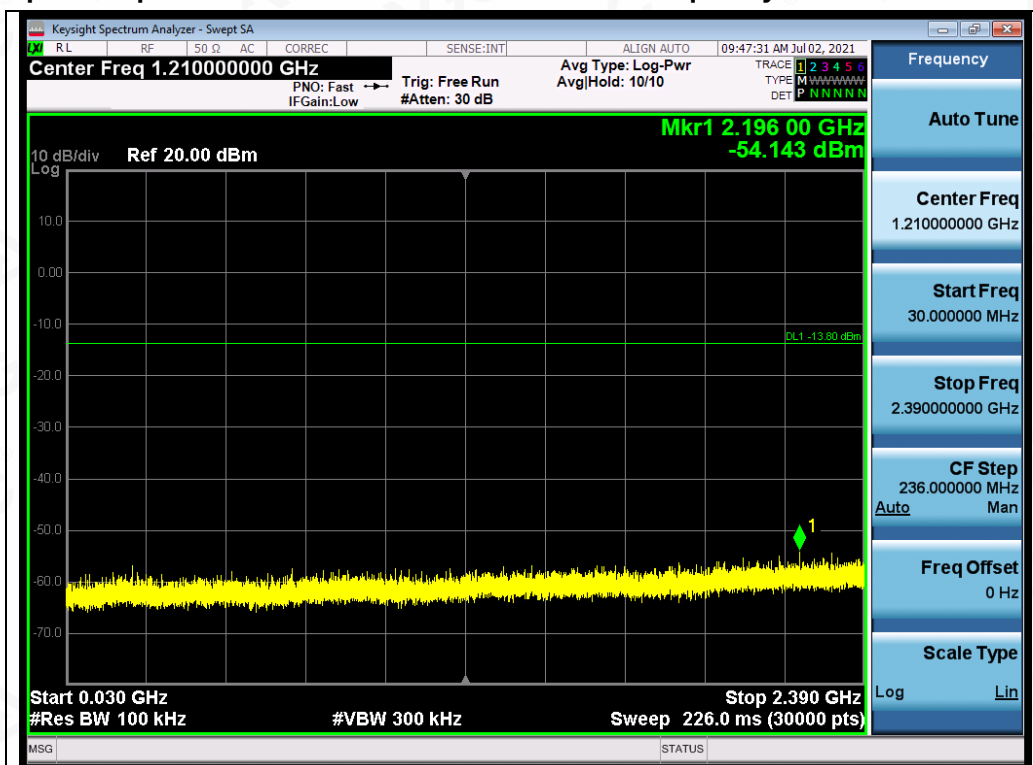
Test_Graph_CCK_ANT1_2412_1Mbps_Lower Band Emissions
