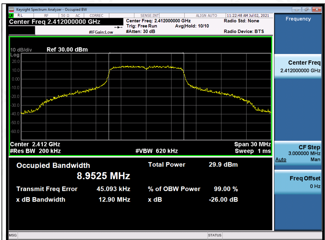
Test_Graph_OFDM_ANT2_2412_MCS0_OBW
