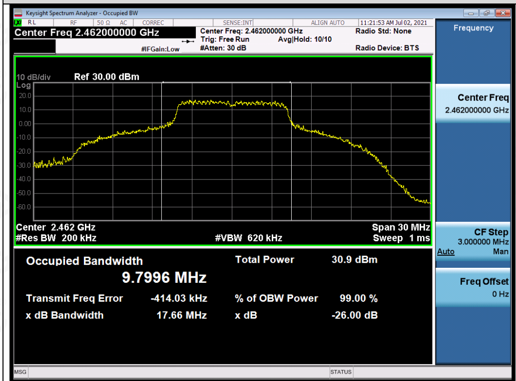
Test_Graph_OFDM_ANT2_2462_6Mbps_OBW
