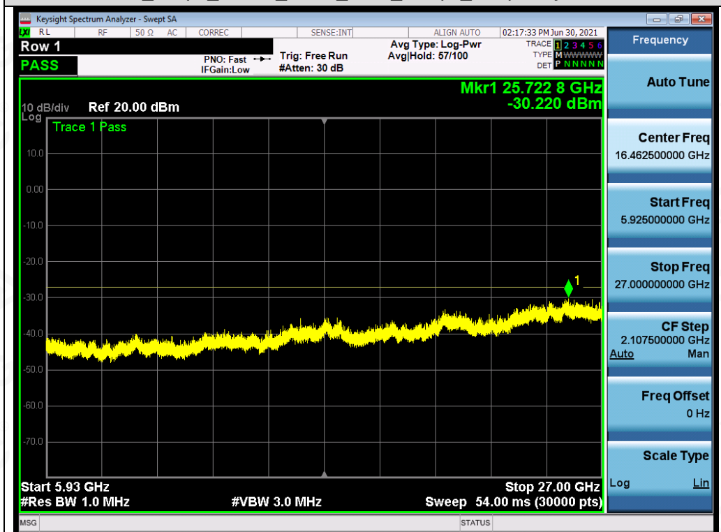
Test_Graph_OFDM_ANT1_5745_6Mbps_Frequency Band4
