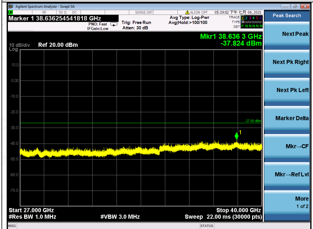
Test_Graph_802.11a_ANT1_5240_6Mbps_Frequency Band 5
