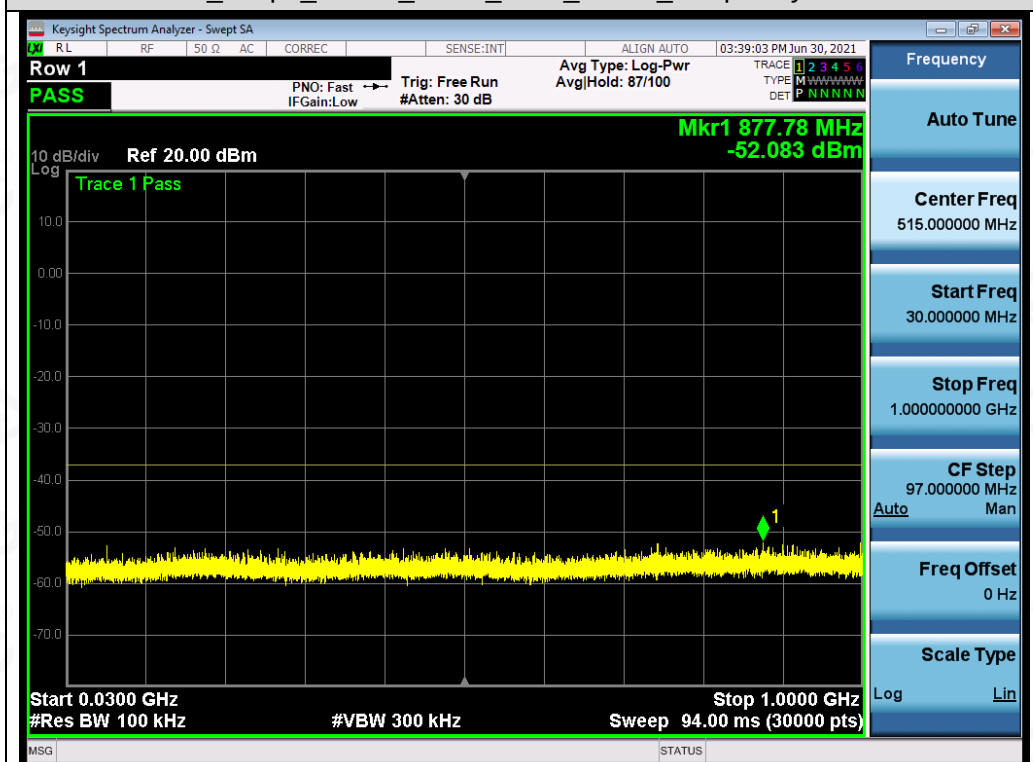
Test_Graph_OFDM_ANT1_5825_MCS0_Frequency Band1
