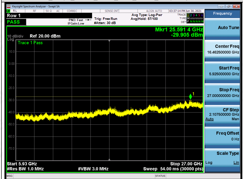
Test_Graph_OFDM_ANT1_5745_MCS0_Frequency Band4
