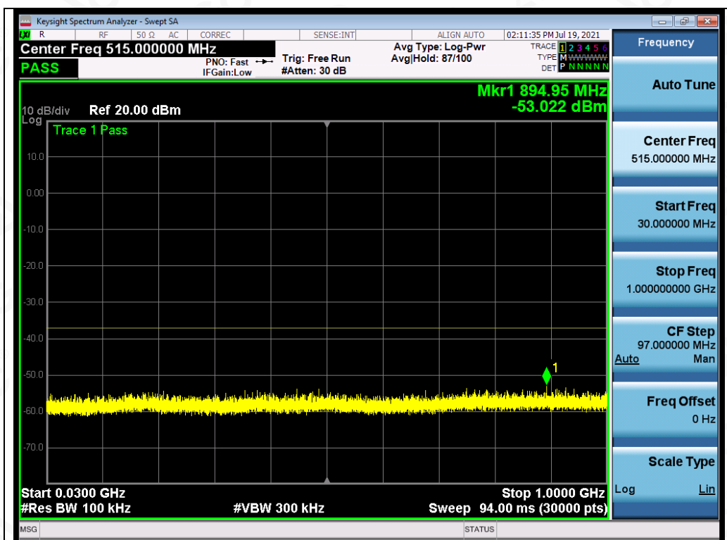
Test_Graph_802.11n20_ANT1_5180_MCS0_Frequency Band 1
