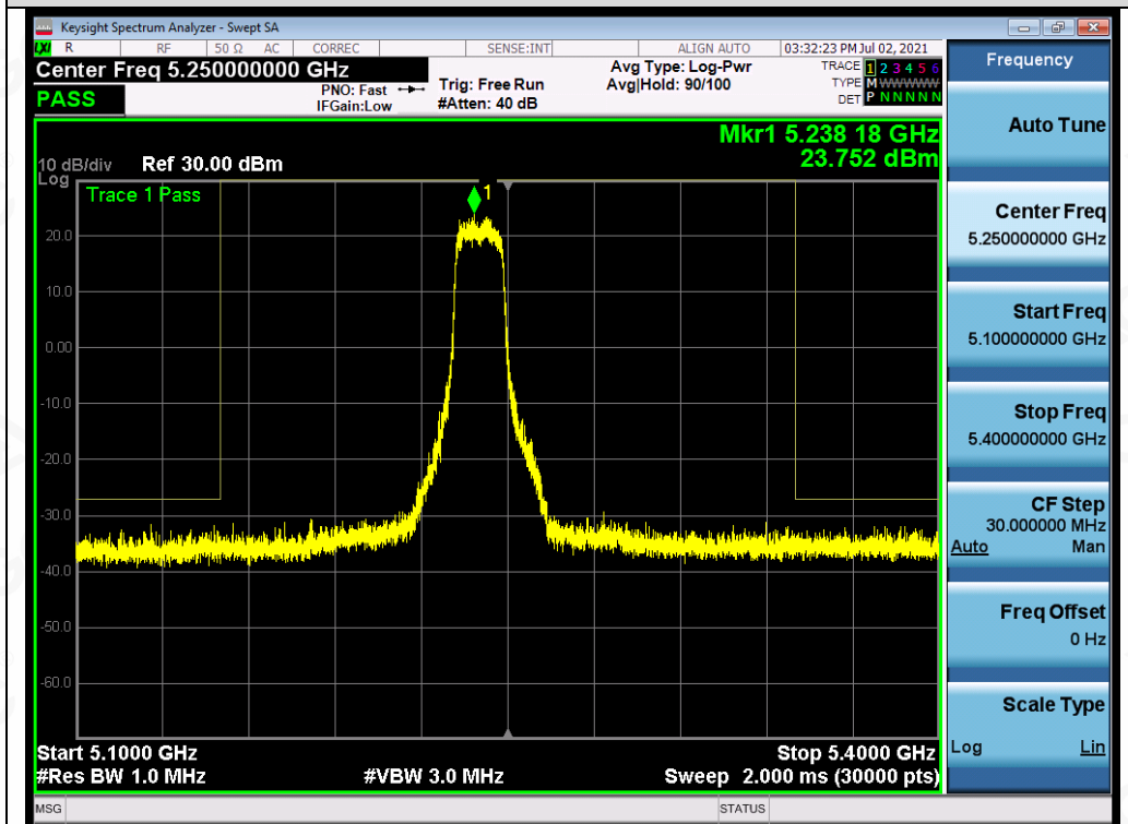
Test_Graph_802.11a_ANT1_5240_6Mbps_Frequency Band 3
