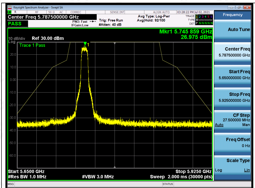
Test_Graph_OFDM_ANT1_5745_MCS0_Frequency Band3
