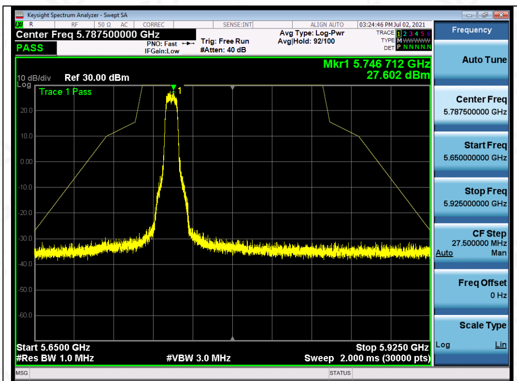
Test_Graph_OFDM_ANT1_5745_6Mbps_Frequency Band3
