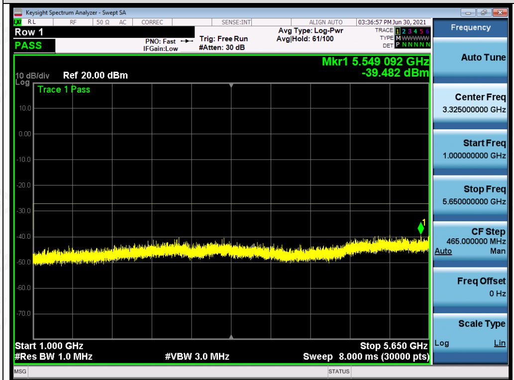
Test_Graph_OFDM_ANT1_5745_MCS0_Frequency Band2
