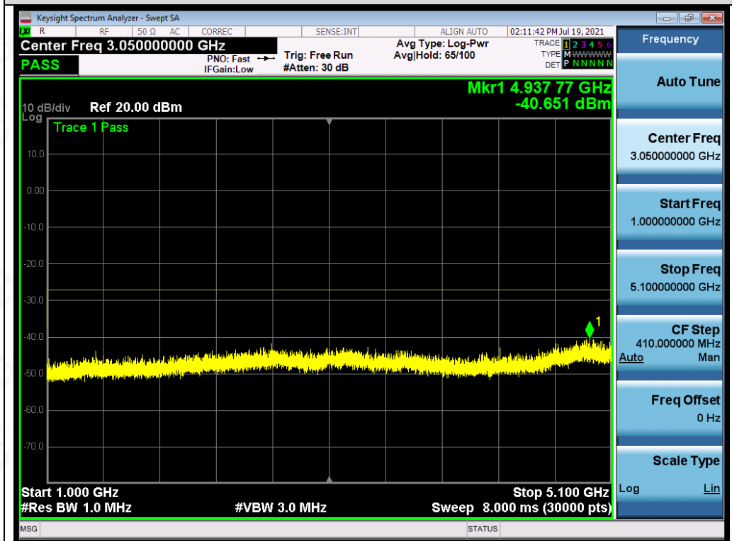
Test_Graph_802.11n20_ANT1_5180_MCS0_Frequency Band 2
