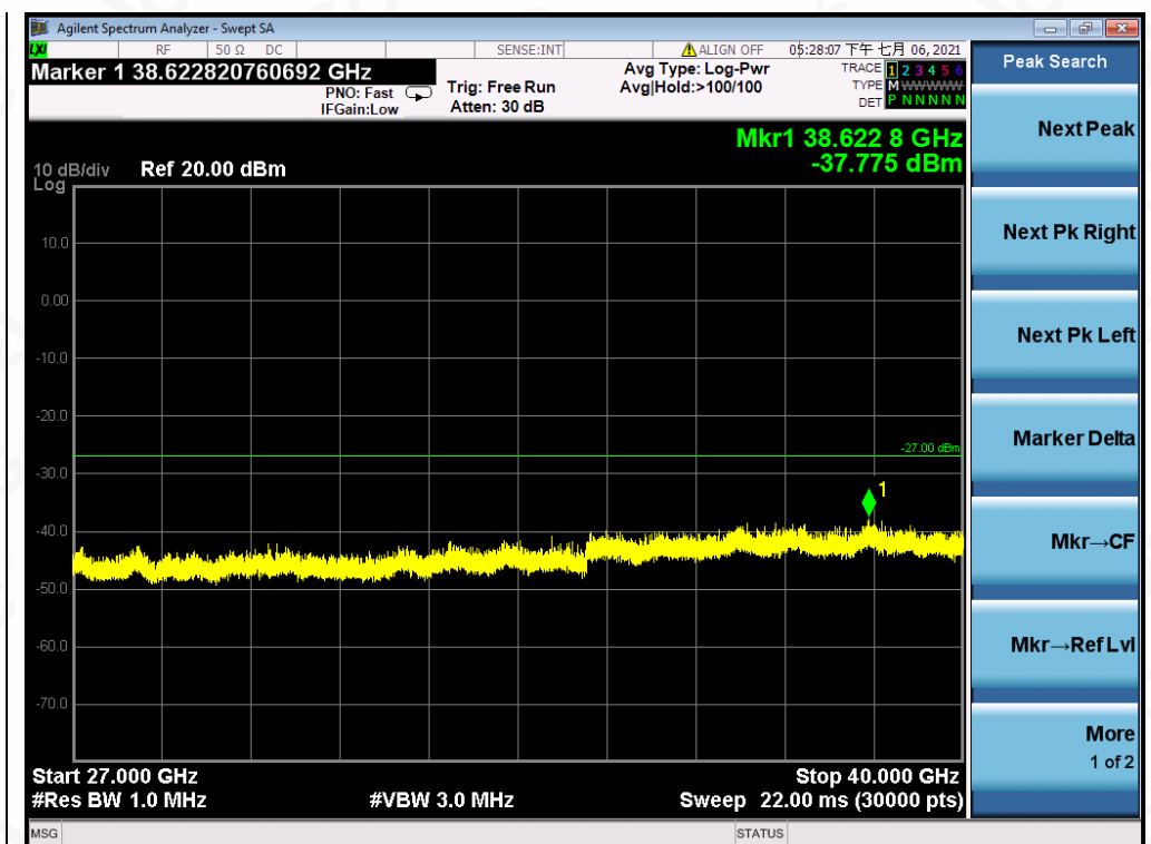
Test_Graph_802.11a_ANT1_5180_6Mbps_Frequency Band 5
