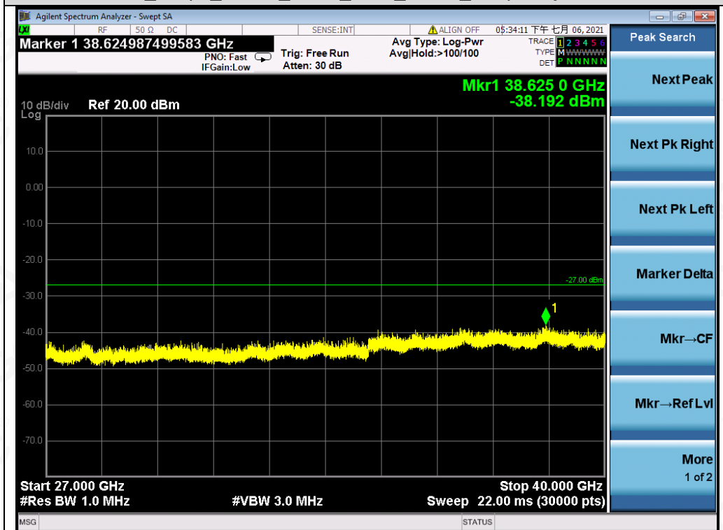
Test_Graph_OFDM_ANT1_5825_MCS0_Frequency Band5
