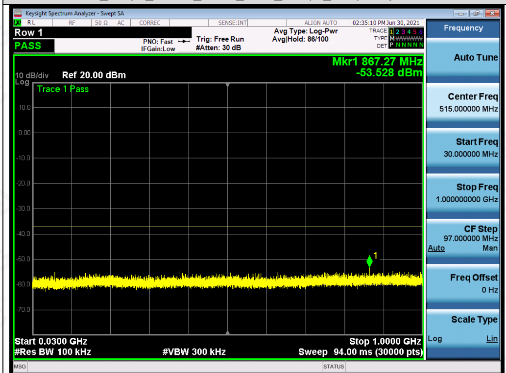
Test_Graph_OFDM_ANT1_5825_6Mbps_Frequency Band1
