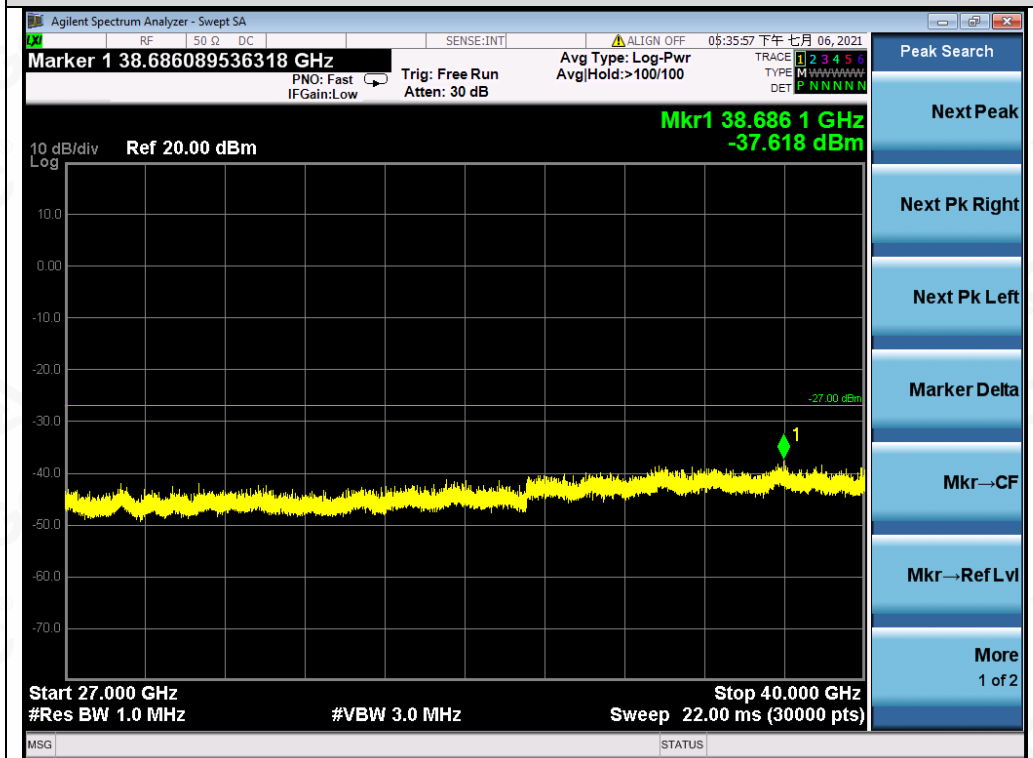
Test_Graph_802.11a_ANT1_5240_6Mbps_Frequency Band 5
