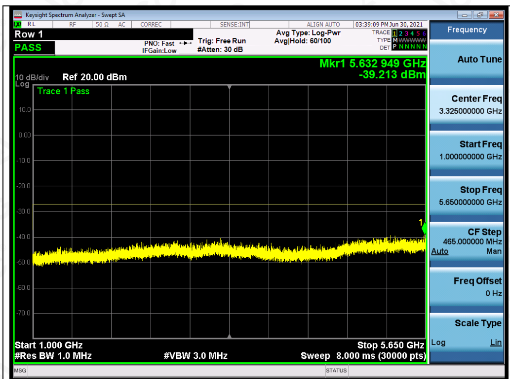
Test_Graph_OFDM_ANT1_5825_MCS0_Frequency Band2
