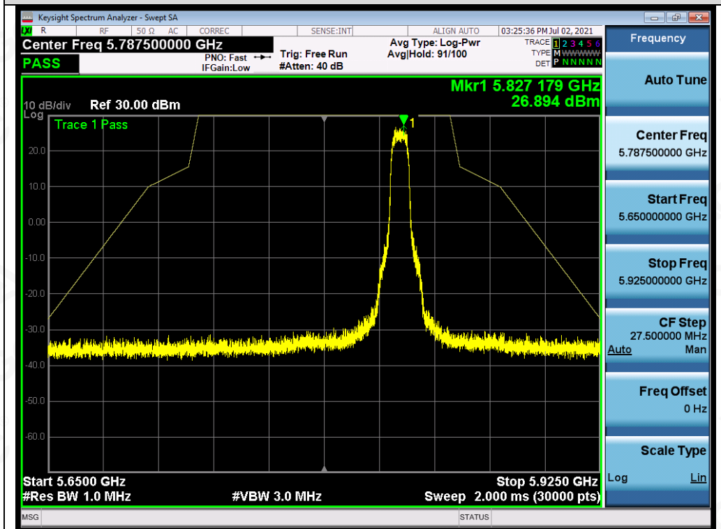
Test_Graph_OFDM_ANT1_5825_6Mbps_Frequency Band3
