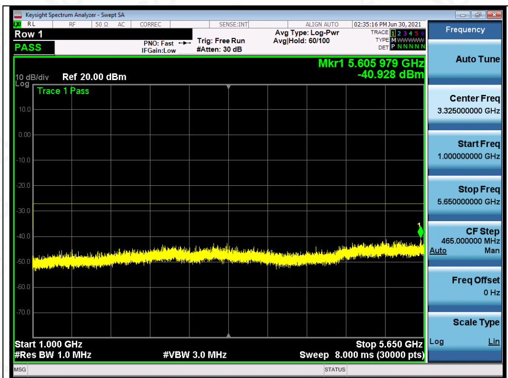
Test_Graph_OFDM_ANT1_5825_6Mbps_Frequency Band2
