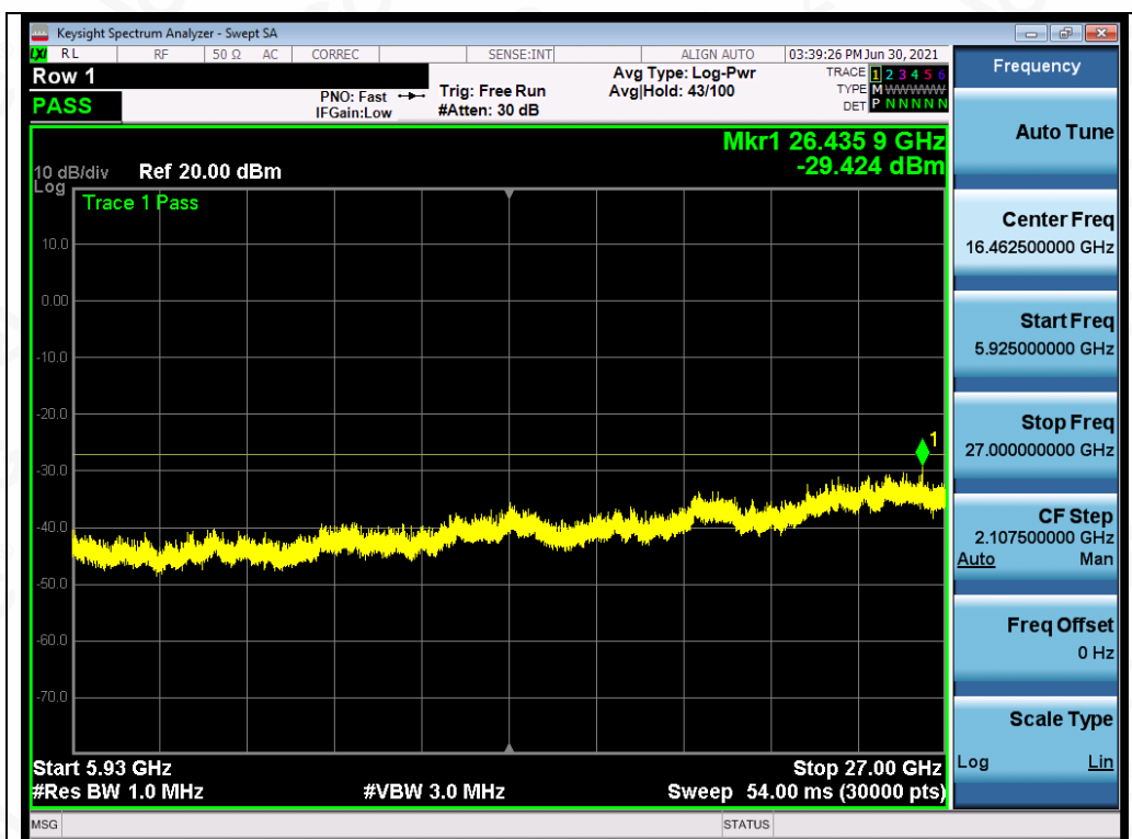
Test_Graph_OFDM_ANT1_5825_MCS0_Frequency Band4
