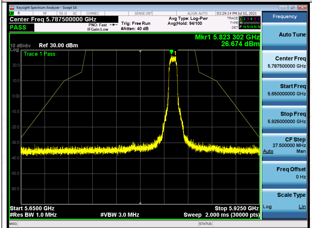
Test_Graph_OFDM_ANT1_5825_MCS0_Frequency Band3
