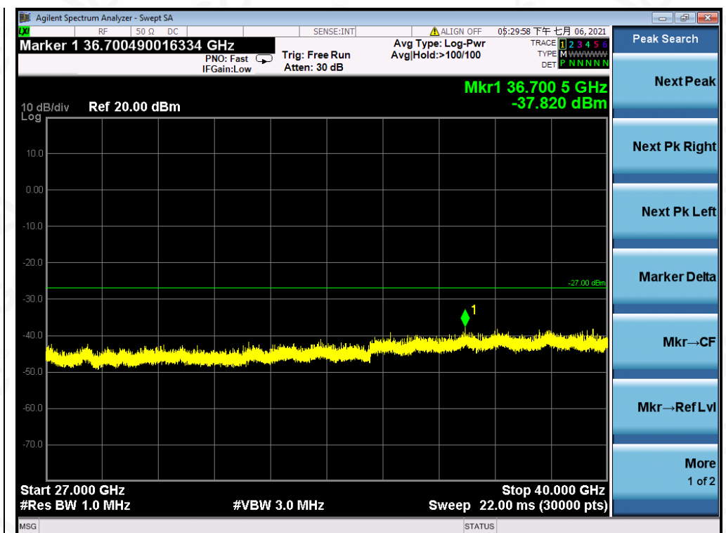
Test_Graph_OFDM_ANT1_5745_6Mbps_Frequency Band5
