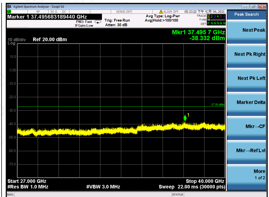
Test_Graph_OFDM_ANT1_5745_MCS0_Frequency Band5
