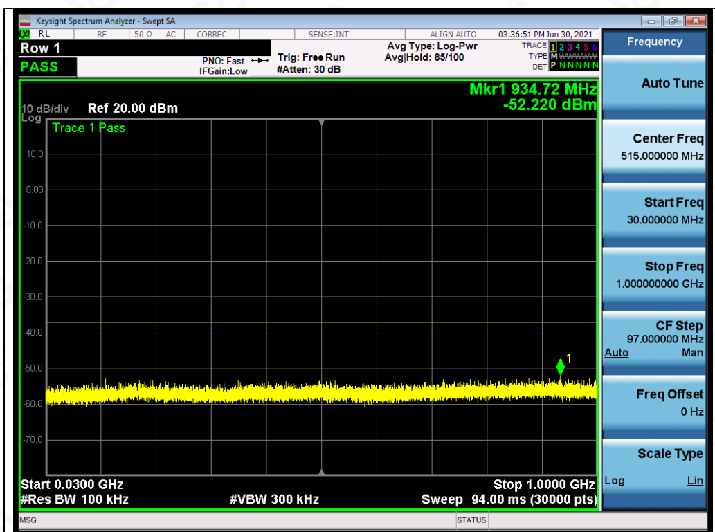
Test_Graph_OFDM_ANT1_5745_MCS0_Frequency Band1
