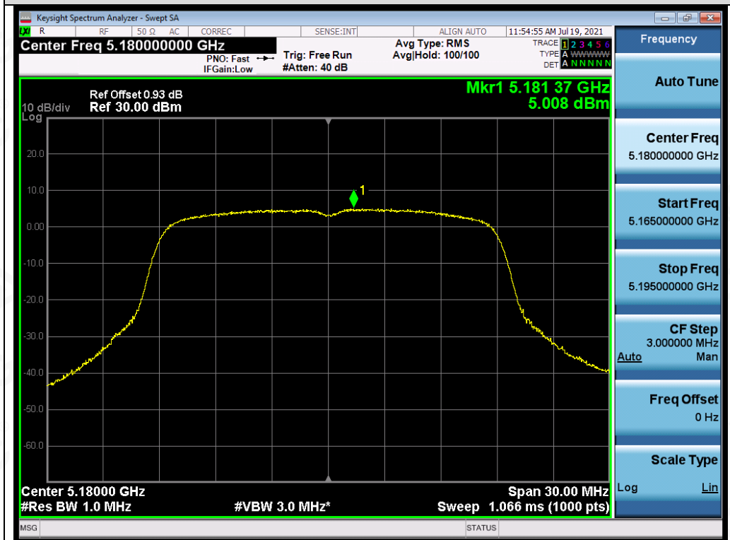
Test_Graph_802.11n20_ANT4_5180_MCS0_PSD
