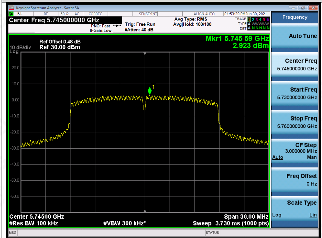
Test_Graph_802.11n20_ANT3_5745_MCS0_PSD
