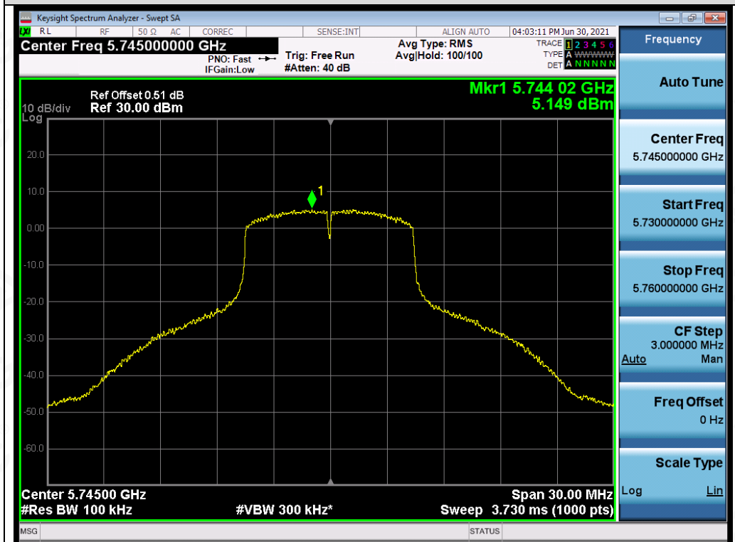
Test_Graph_OFDM_ANT3_5745_MCS0_PSD
