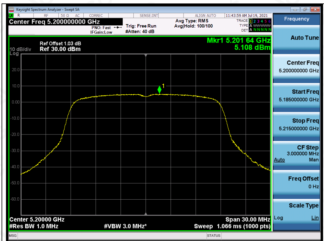
Test_Graph_802.11n20_ANT3_5200_MCS0_PSD
