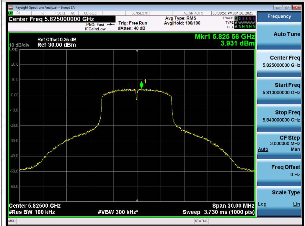
Test_Graph_OFDM_ANT1_5825_MCS0_PSD
