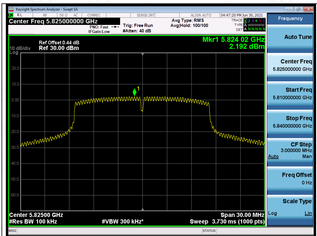
Test_Graph_802.11a_ANT3_5825_6Mbps_PSD
