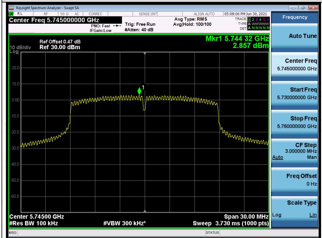
Test_Graph_802.11n20_ANT4_5745_MCS0_PSD
