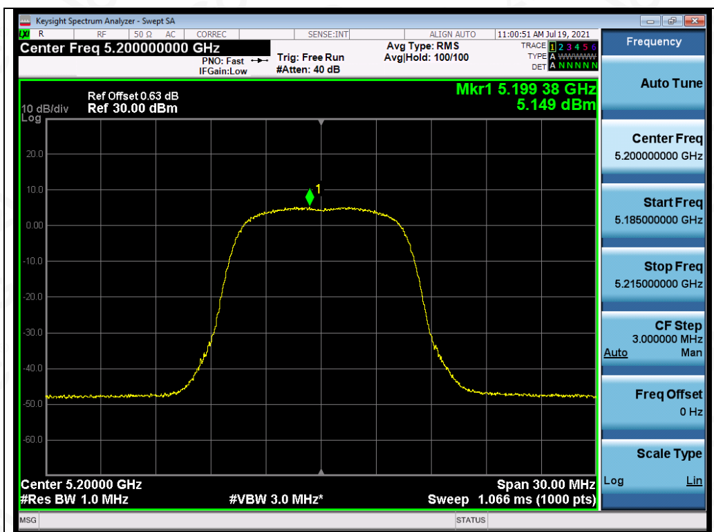
Test_Graph_OFDM_ANT4_5200_MCS0_PSD
