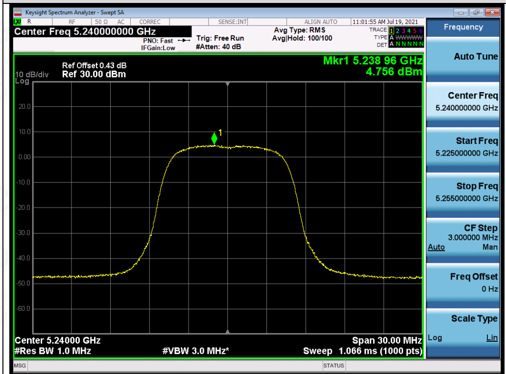
Test_Graph_OFDM_ANT4_5240_MCS0_PSD
