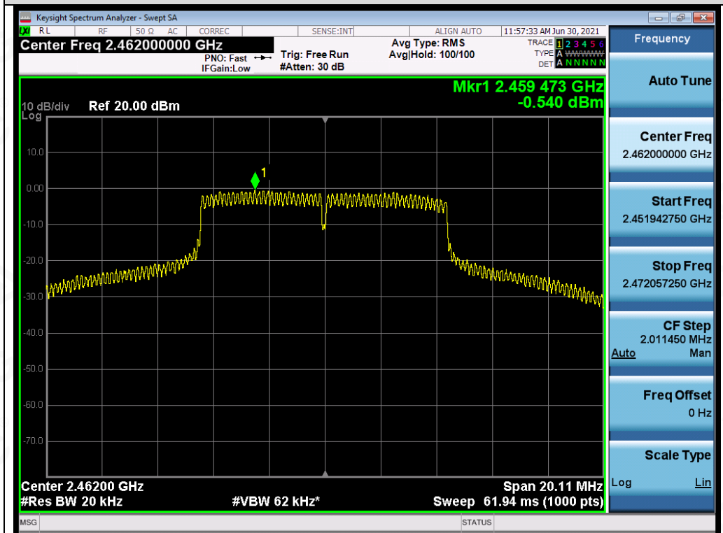
Test_Graph_OFDM_ANT4_2462_MCS0_PSD
