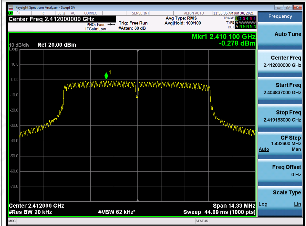
Test_Graph_OFDM_ANT4_2412_MCS0_PSD
