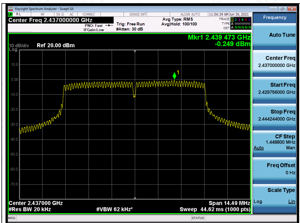
Test_Graph_OFDM_ANT4_2437_MCS0_PSD
