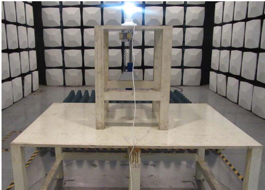
Radiated Disturbance Test Setup Front View (Above 1GHz)
