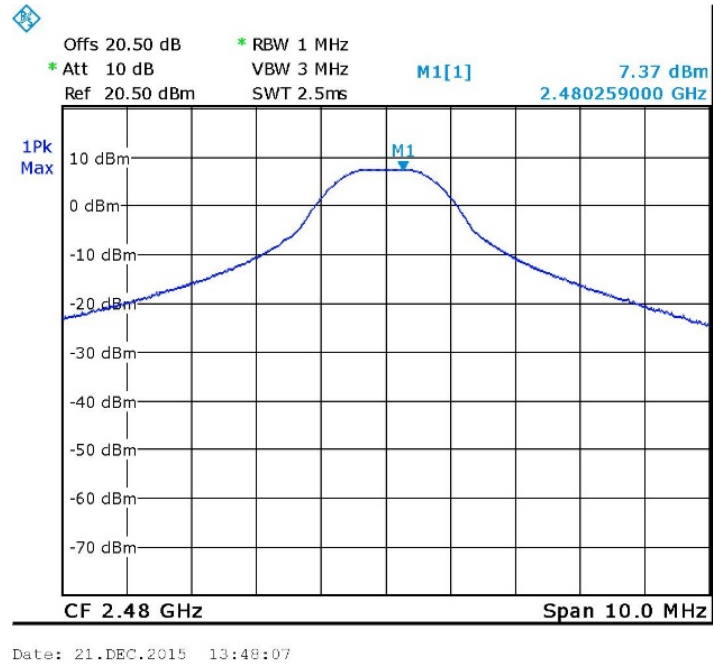
Figure 23 2480.0 MHz
