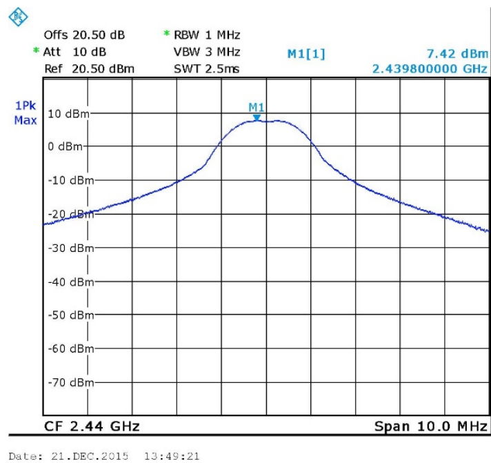
Figure 22 2440.0 MHz
