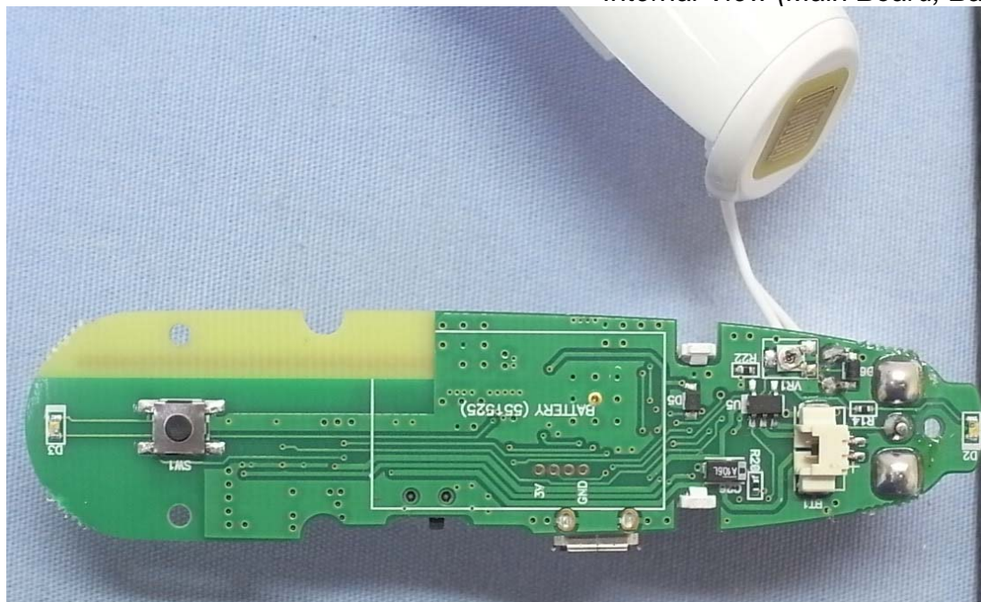
Figure 10 Internal View (Main Board, Back View)
