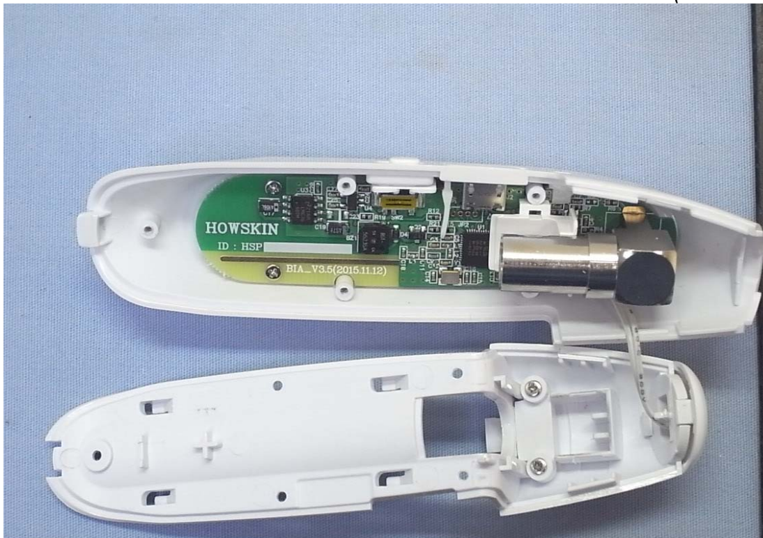
Figure 6 Internal View (Removed Cover)
