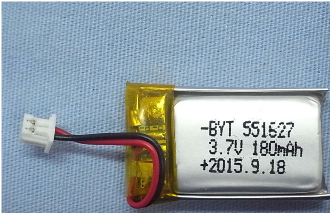
Figure 8 Internal View (Battery)
