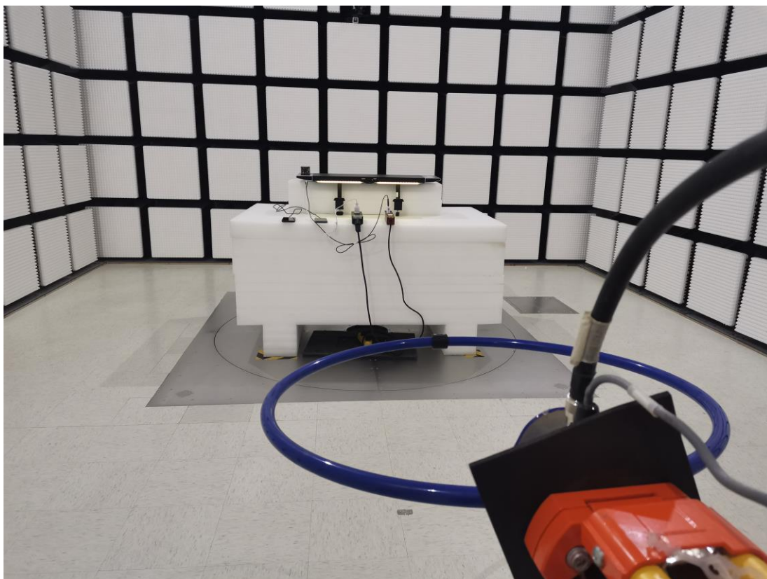
Radiated Emission 9kHz~30MHz Ground-parallel Rear View
