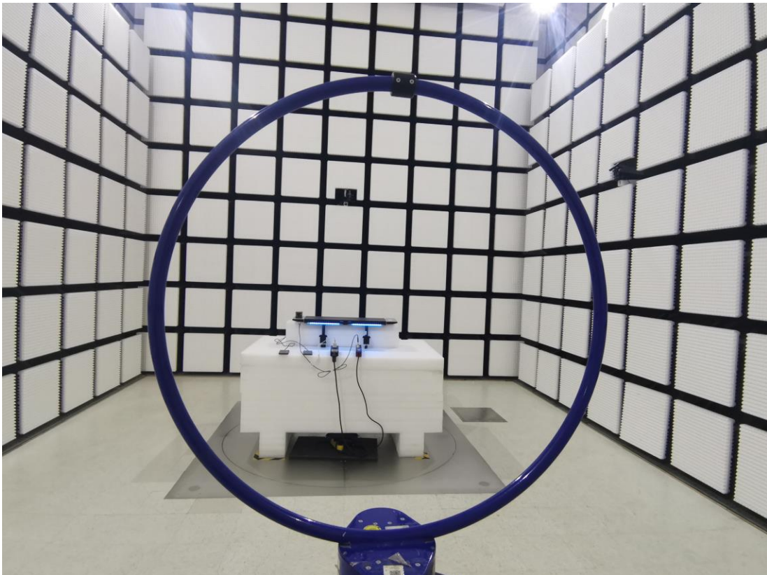
Radiated Emission 9kHz~30MHz Parallel Rear View
