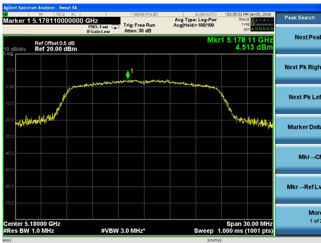
Test Plot For 802.11n(HT20)-5180M
