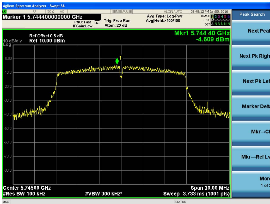
Test Plot For 802.11n(HT20)-5745M
