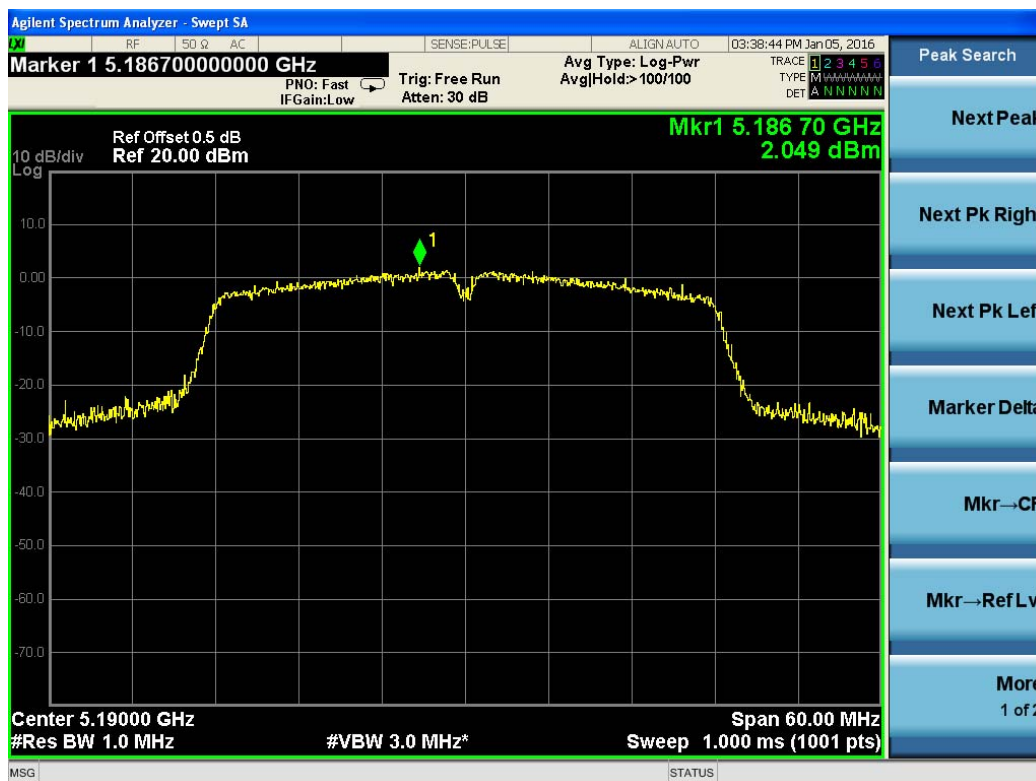
Test Plot For 802.11ac(VHT40)-5190M
