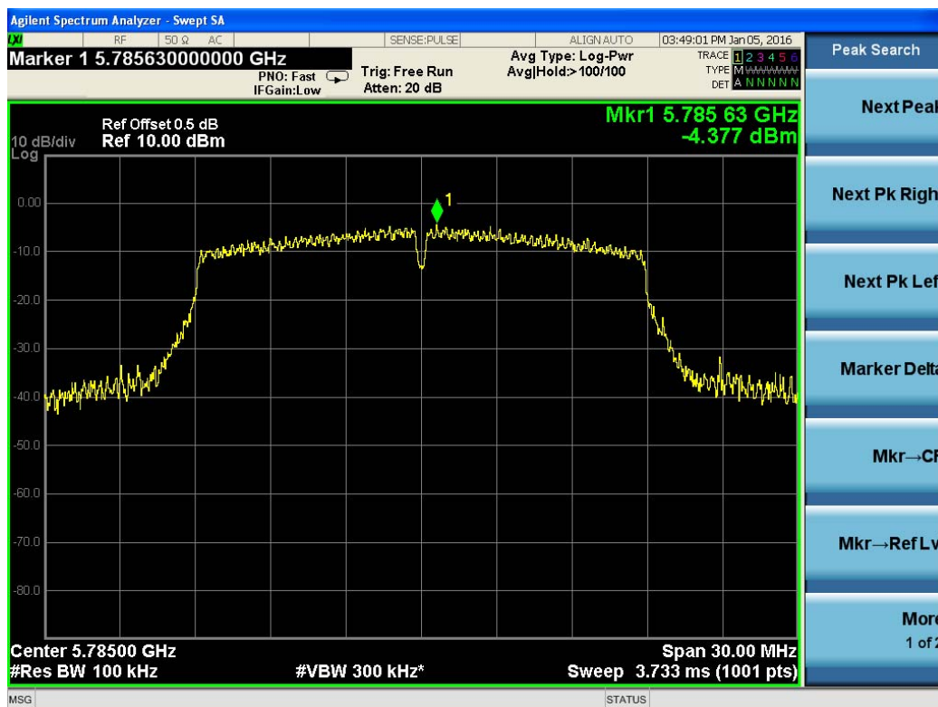
Test Plot For 802.11ac(VHT20)-5785M
