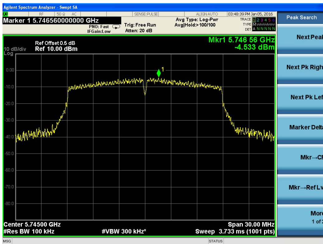
Test Plot For 802.11ac(VHT20)-5745M
