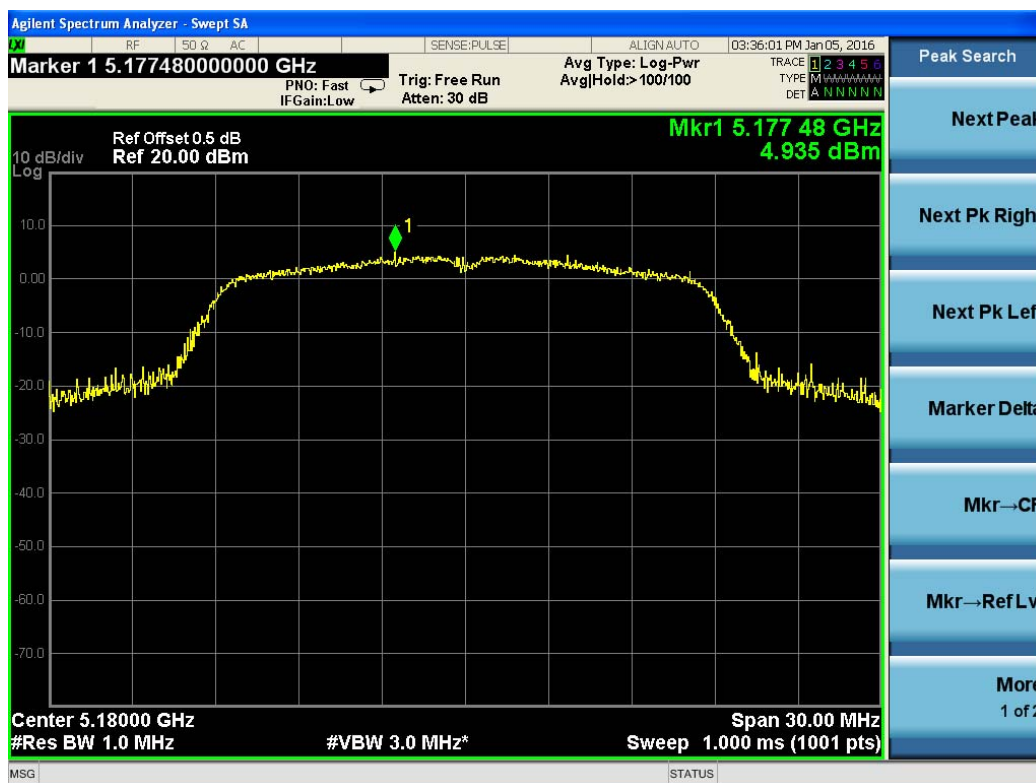
Test Plot For 802.11ac(VHT20)-5180M
