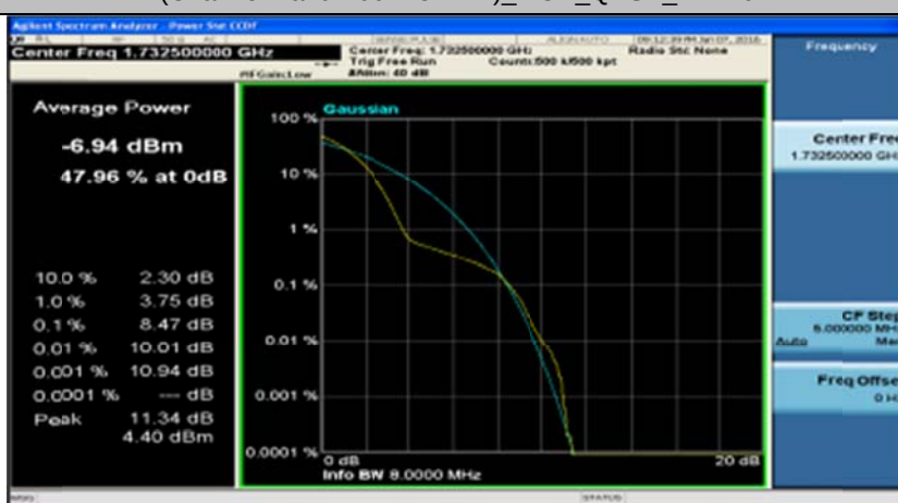
(Channel Bandwidth 15 MHz)_MCH_QPSK_1RB#37
