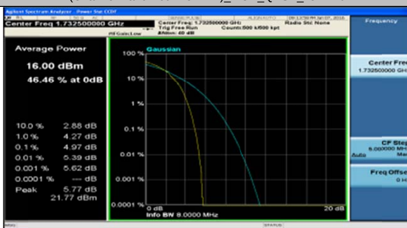
(Channel Bandwidth 15 MHz)_MCH_QPSK_75RB#0
