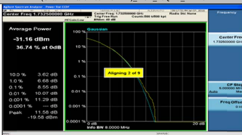
(Channel Bandwidth 20 MHz)_MCH_16QAM_1RB#49
