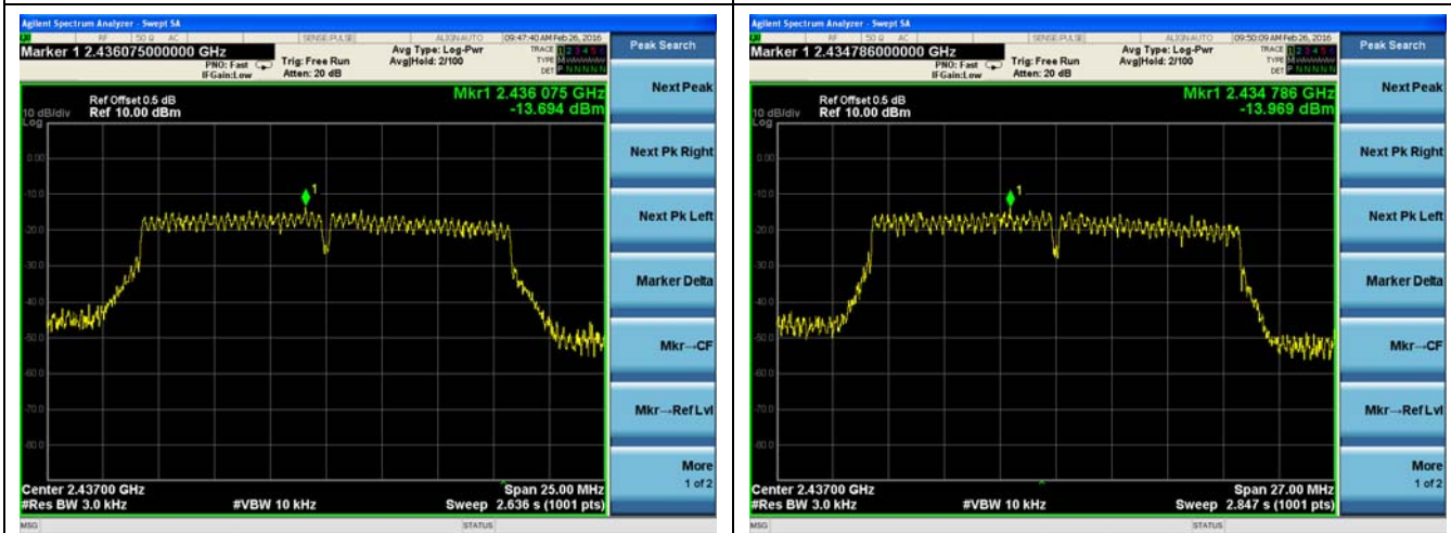
802.11g Middle Channel / 2437MHz
