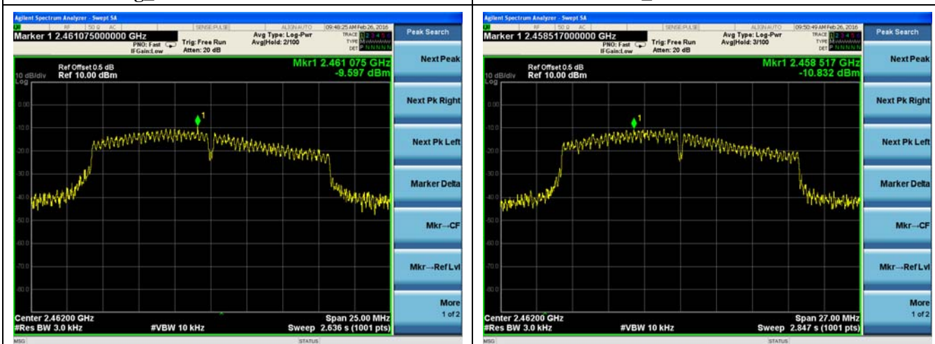
802.11g High Channel / 2462MHz
