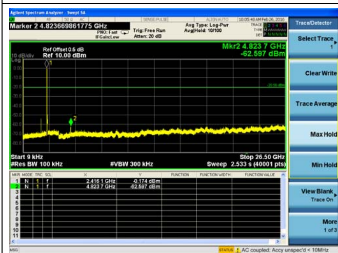
802.11g Low Channel / 2412MHz
