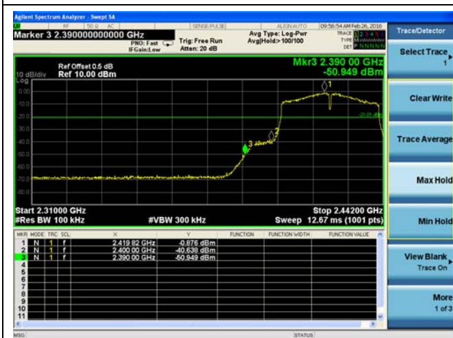
802.11n HT40 Low Channel / 2422MHz
