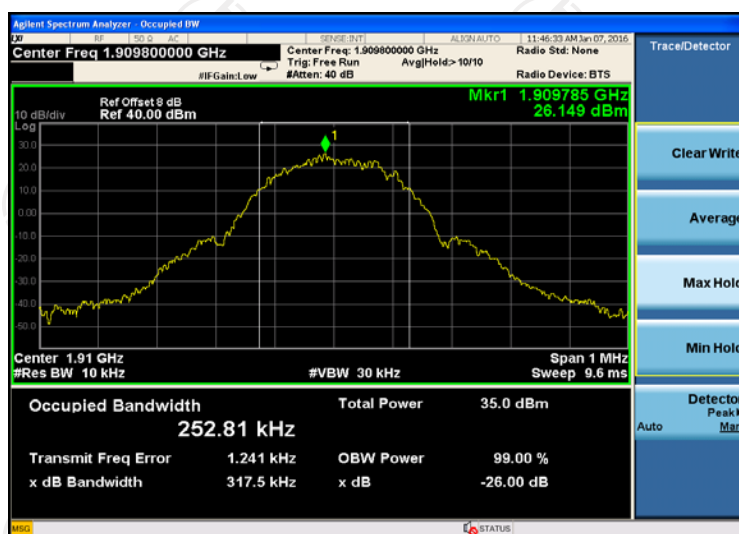
26dB bandwidth Plot on Channel 810
