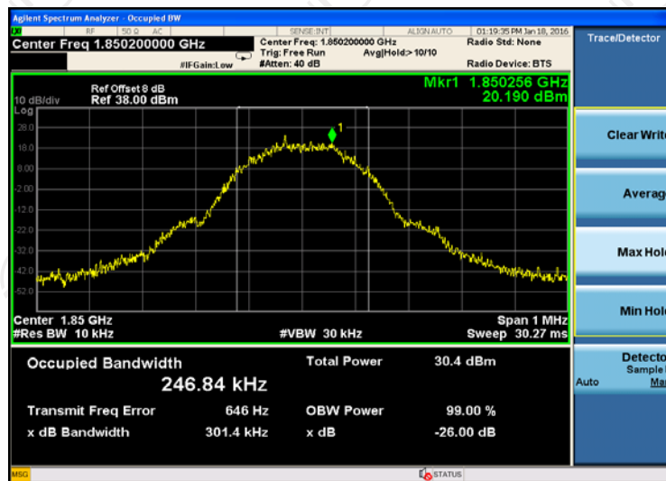
26dB bandwidth Plot on Channel 512
