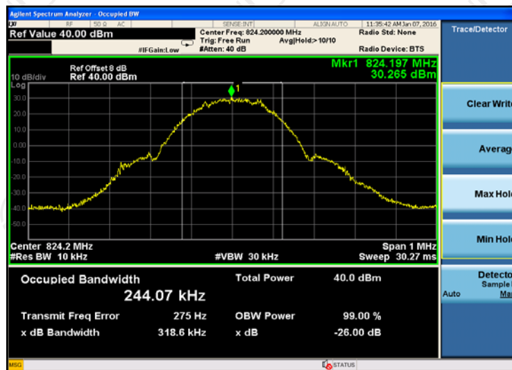
26dB bandwidth Plot on Channel 128
