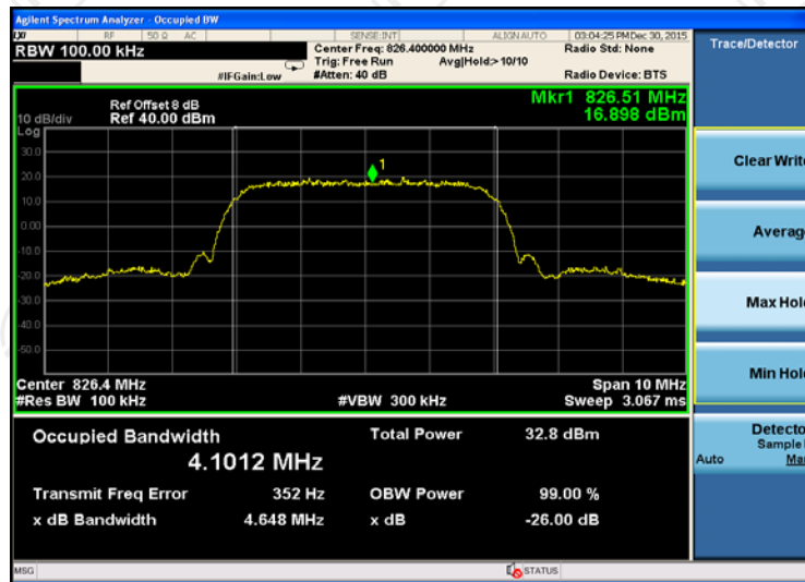
26dB bandwidth Plot on Channel 4132
