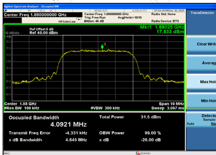
99%Occupied Bandwidth Plot on Channel 9400
