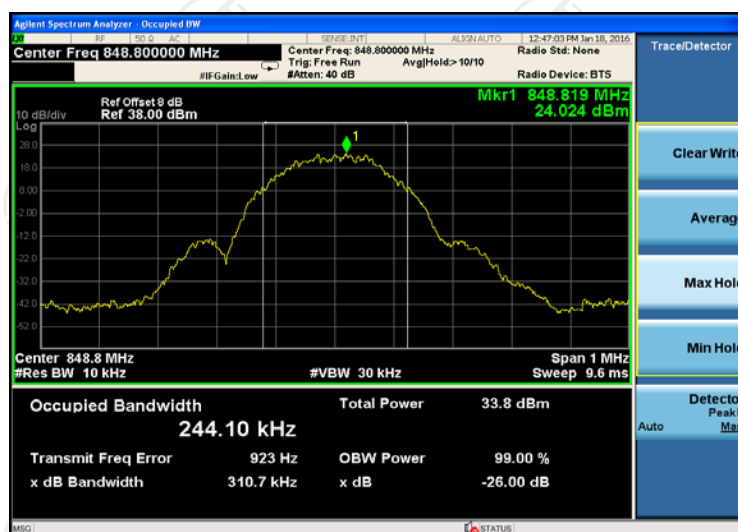
26dB bandwidth Plot on Channel 251
