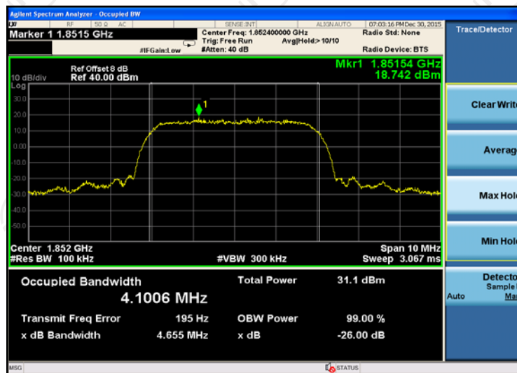
26dB bandwidth Plot on Channel 9262
