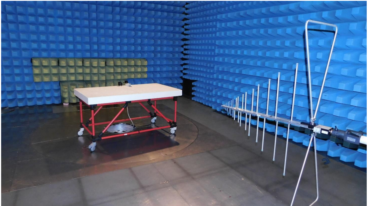
Picture 4: SAC, radiated emission test 30 MHz - 1 GHz (rear view), charging mode
