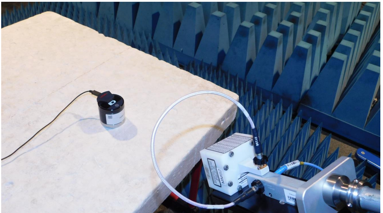
Picture 6: FS-SAC, exploratory radiated emission test 17 GHz - 25 GHz, charging mode
