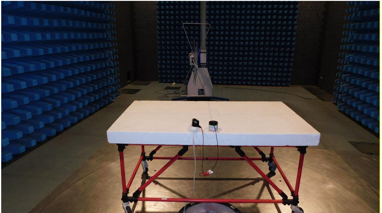
Picture 3: SAC, radiated emission test 30 MHz - 1 GHz (front view), charging mode
