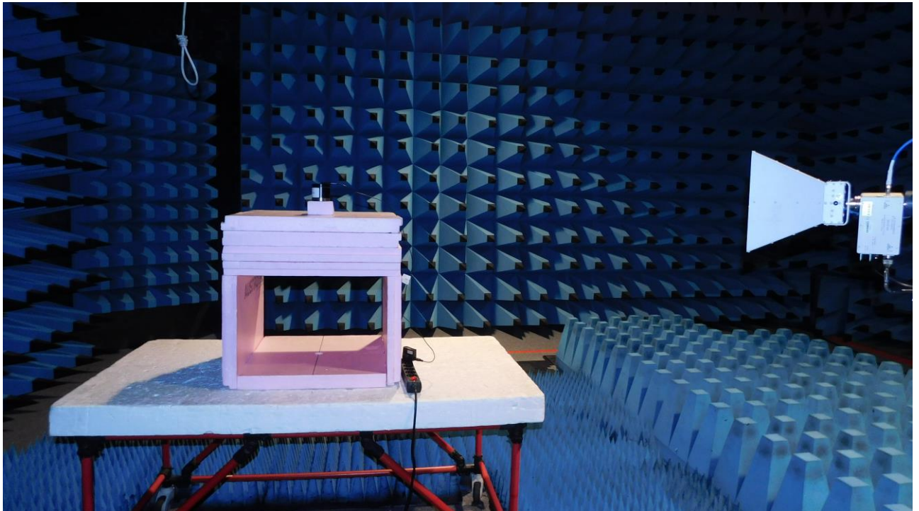
Picture 5: FS-SAC, radiated emission test 1 GHz - 17 GHz, charging mode
